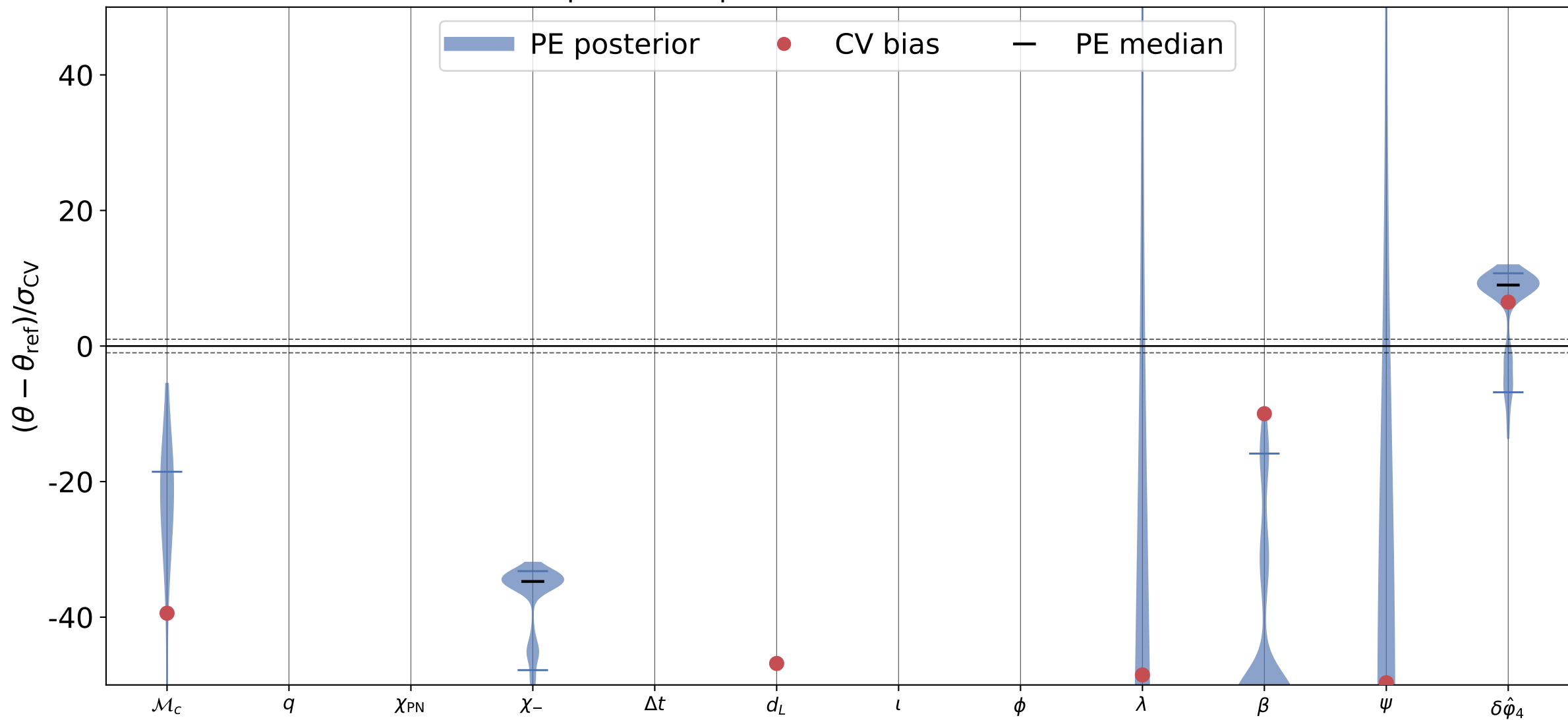
\delta\hat{\phi}_4 recovery, inj_id = 0 processed posterior; reference = truth
