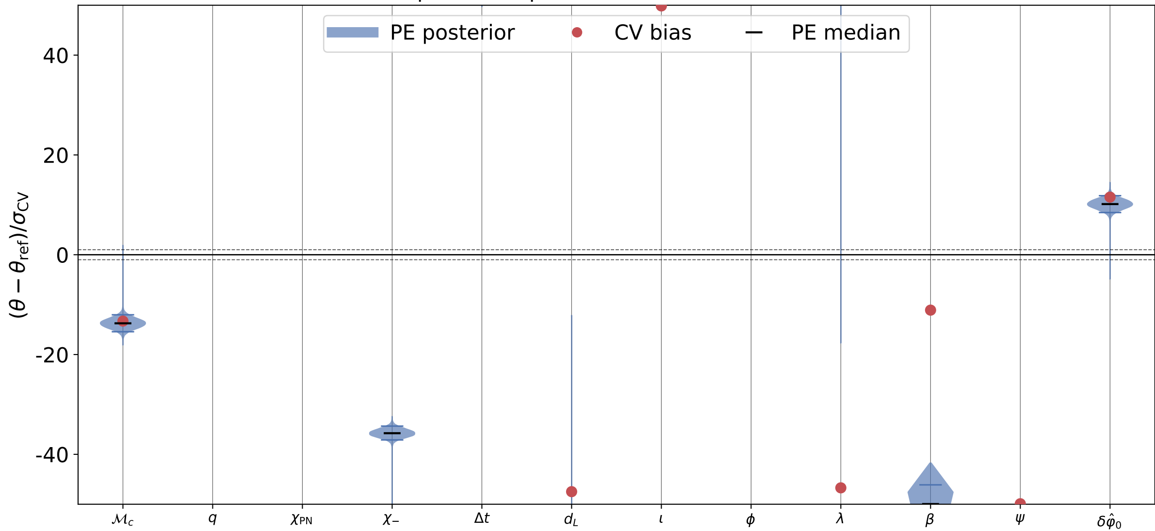
\delta\hat{\phi}_0 recovery, inj_id = 0 processed posterior; reference = truth
