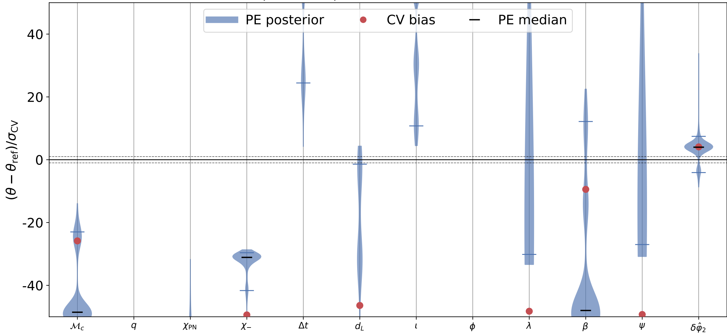
\delta\hat{\phi}_2 recovery, inj_id = 0 processed posterior; reference = truth
