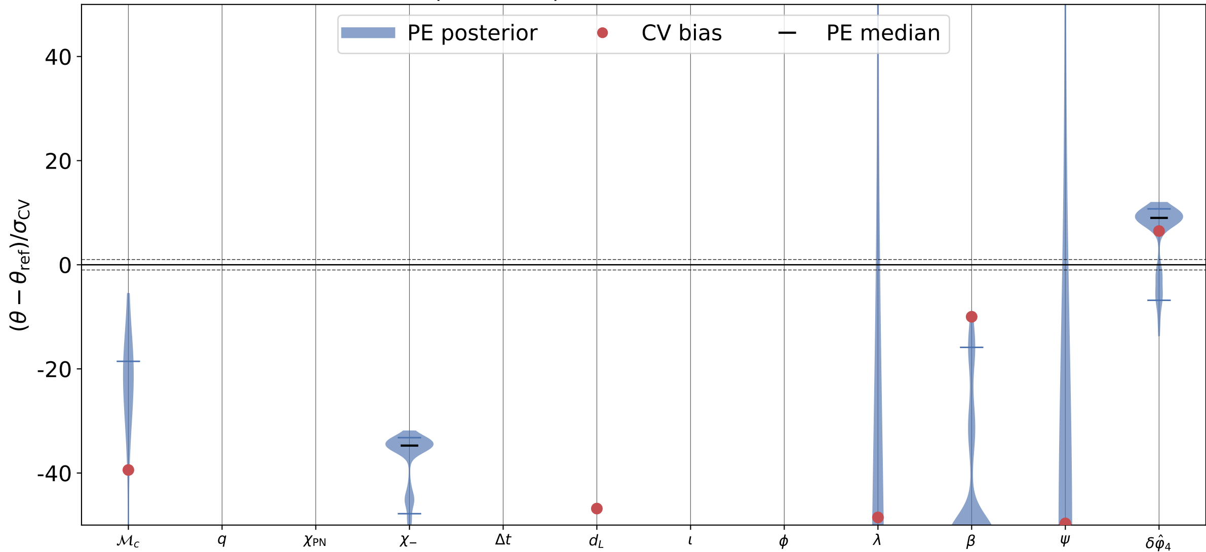
\delta\hat{\phi}_4 recovery, inj_id = 0 processed posterior; reference = truth
