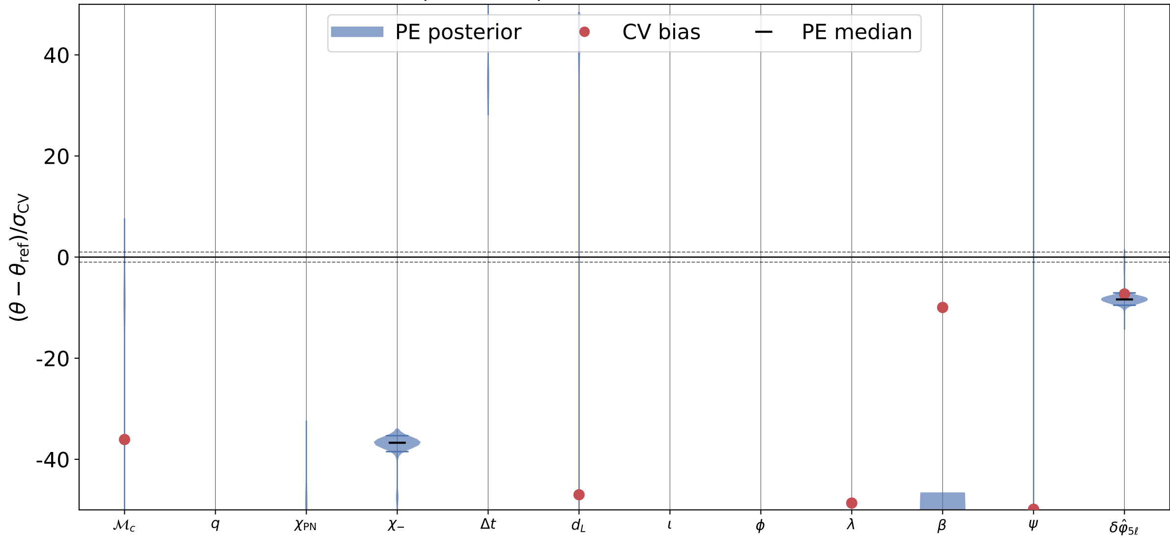
\delta\hat{\phi}_{5\ell} recovery, inj_id = 0 processed posterior; reference = truth
