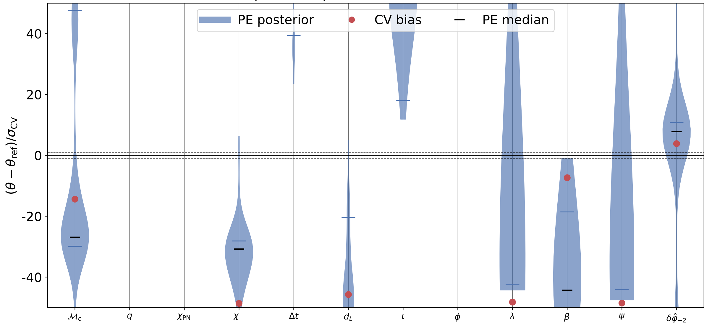
\delta\hat{\phi}_{-2} recovery, inj_id = 0 processed posterior; reference = truth
