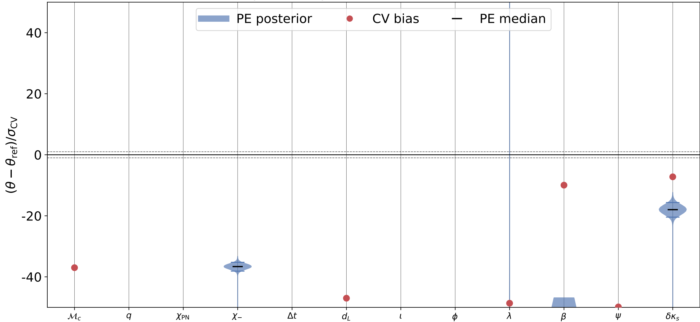
\delta\kappa_s recovery, inj_id = 0 processed posterior; reference = truth
