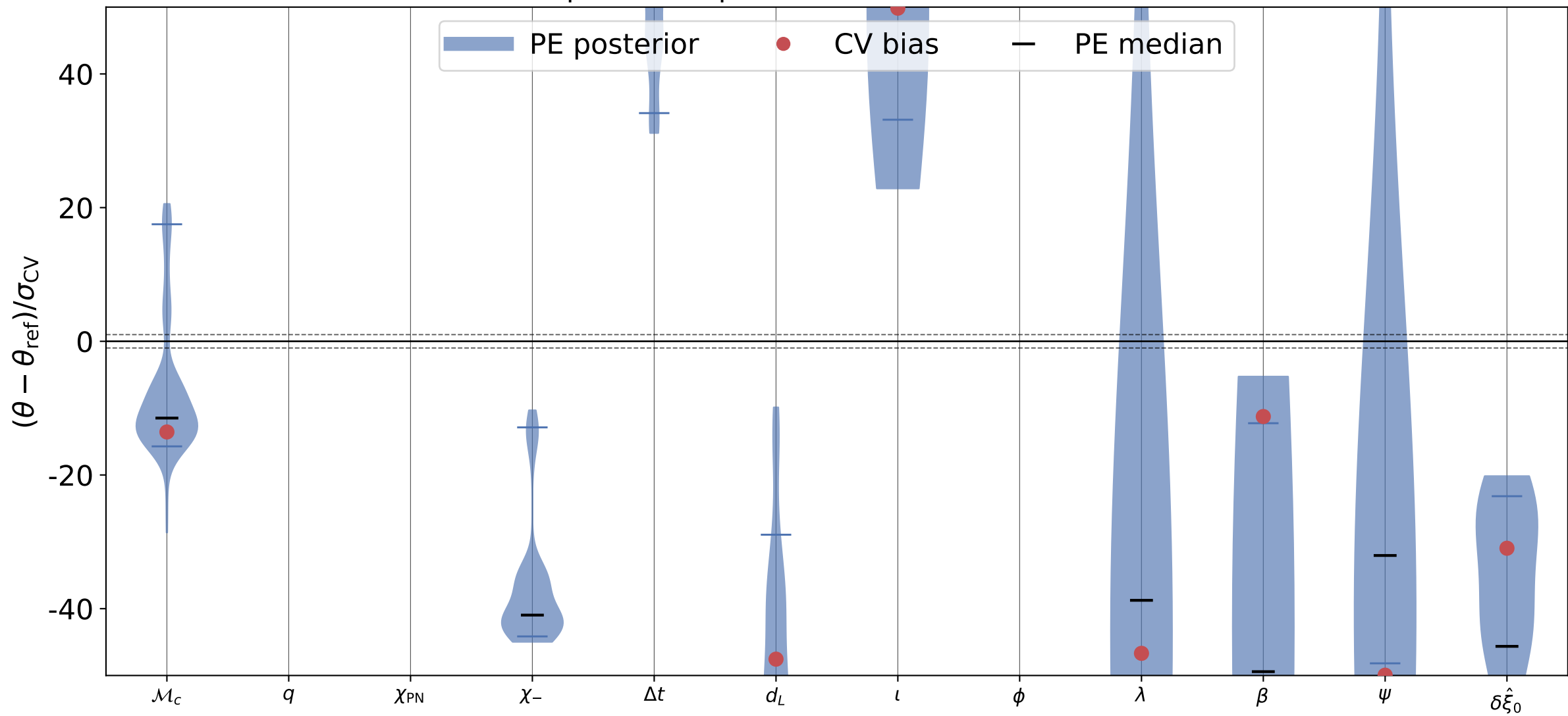
\hat{\delta\xi}_0 recovery, inj_id = 0 processed posterior; reference = truth
