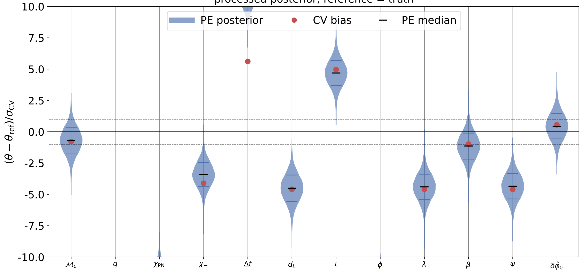
\delta\hat{\phi}_0 recovery, inj_id = 1 processed posterior; reference = truth
