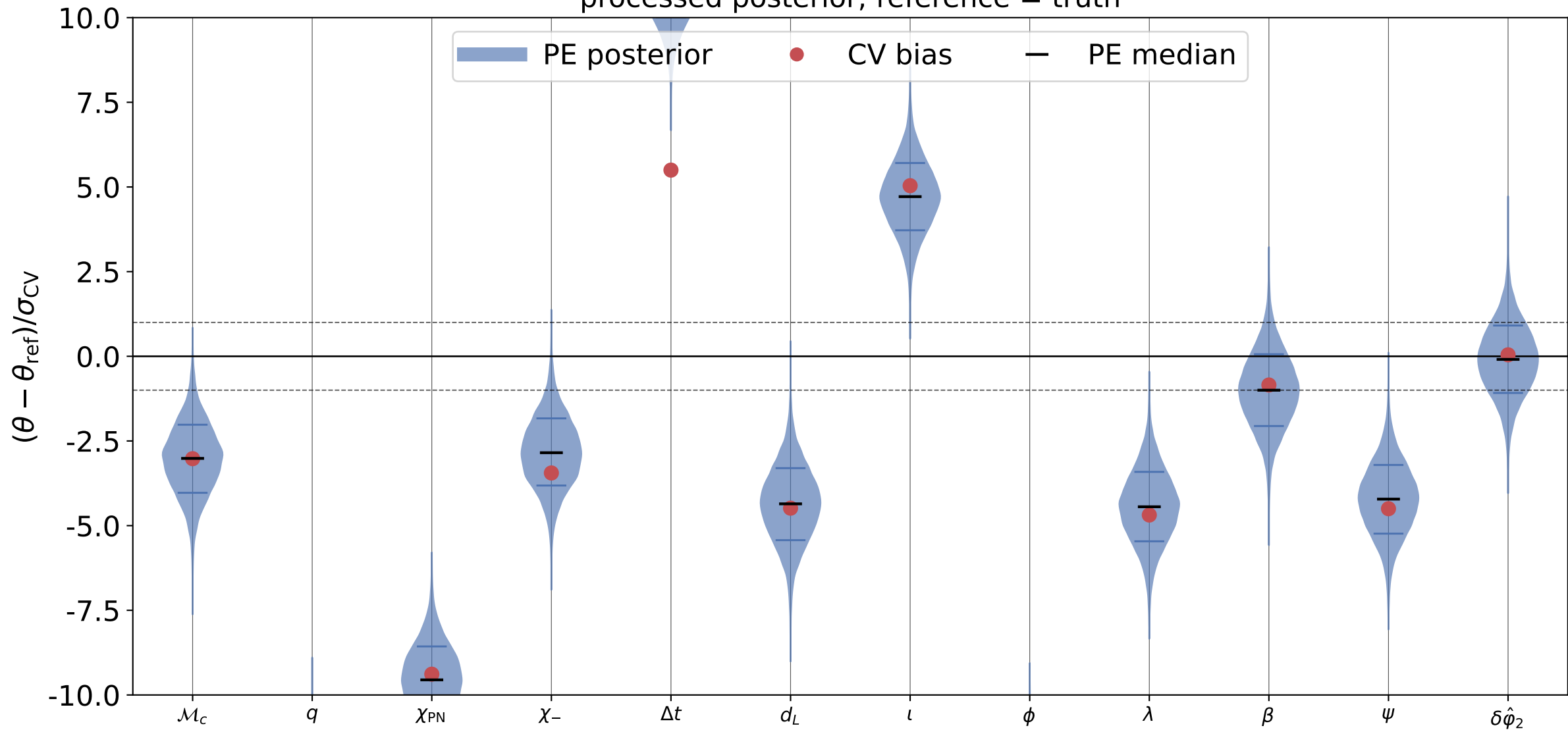
\delta\hat{\phi}_2 recovery, inj_id = 1 processed posterior; reference = truth
