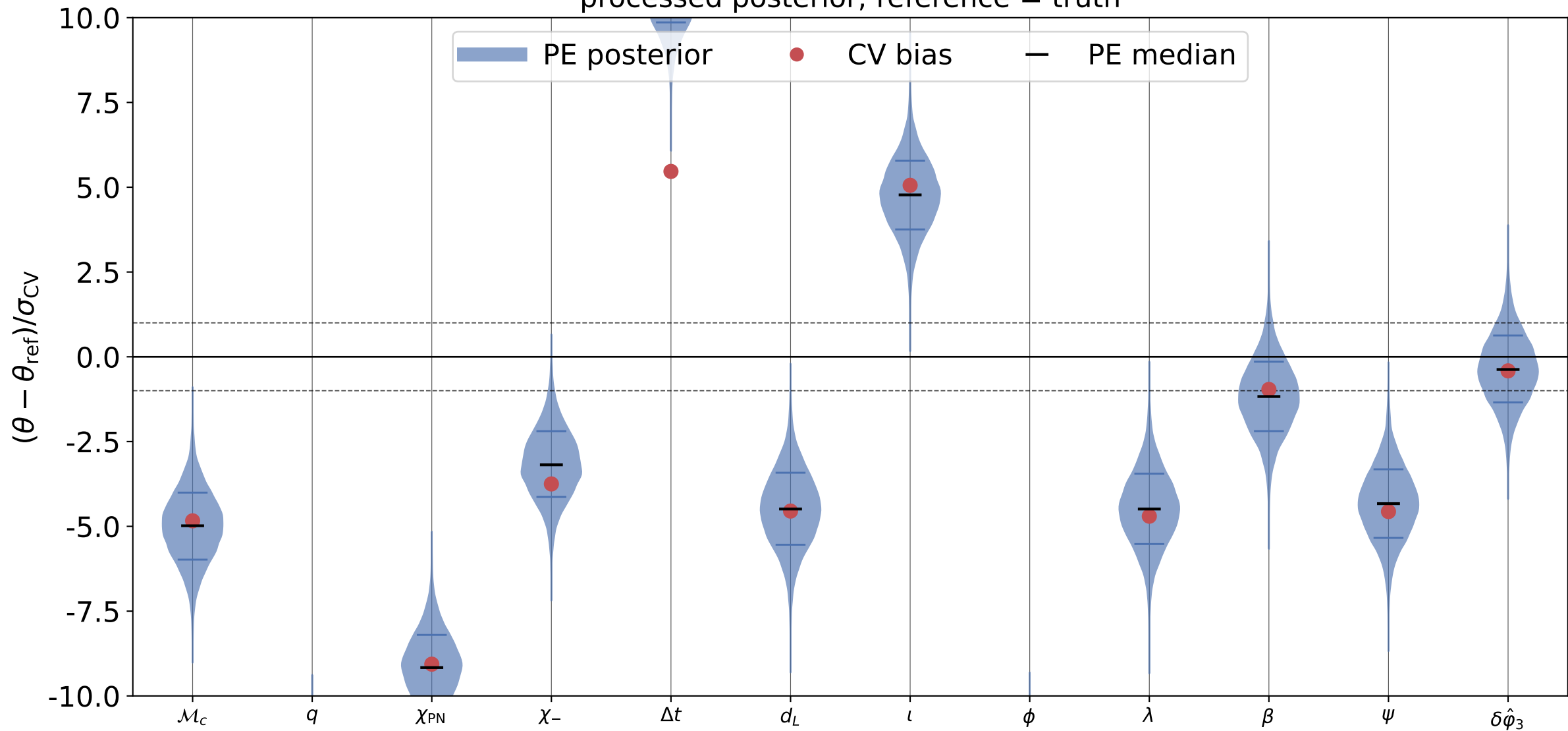
\delta\hat{\phi}_3 recovery, inj_id = 1 processed posterior; reference = truth
