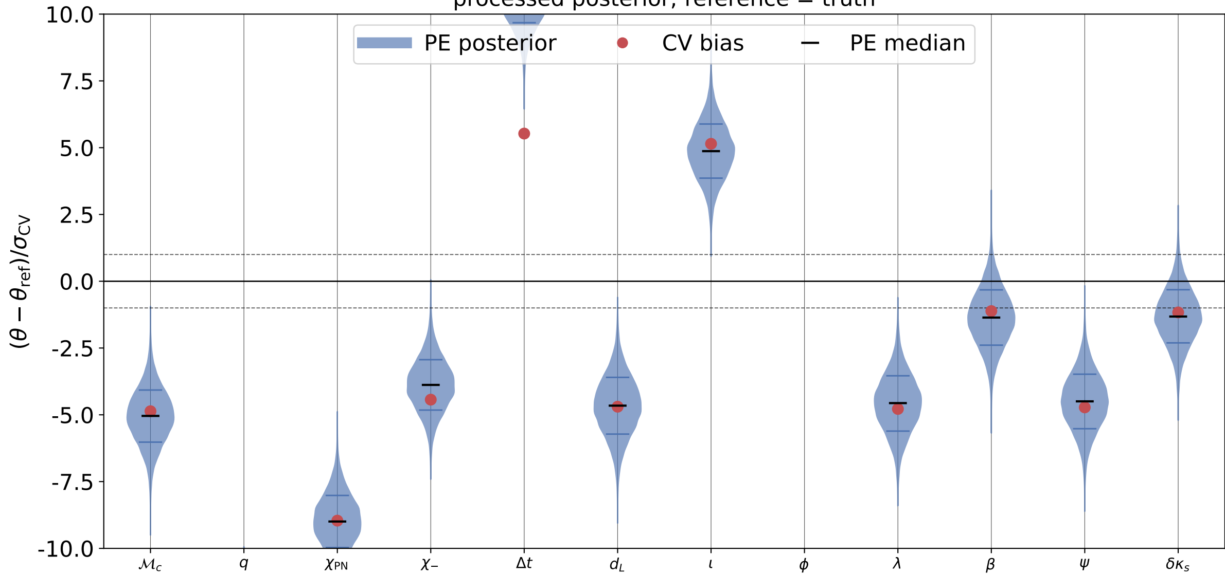
\delta\kappa_s recovery, inj_id = 1 processed posterior; reference = truth
