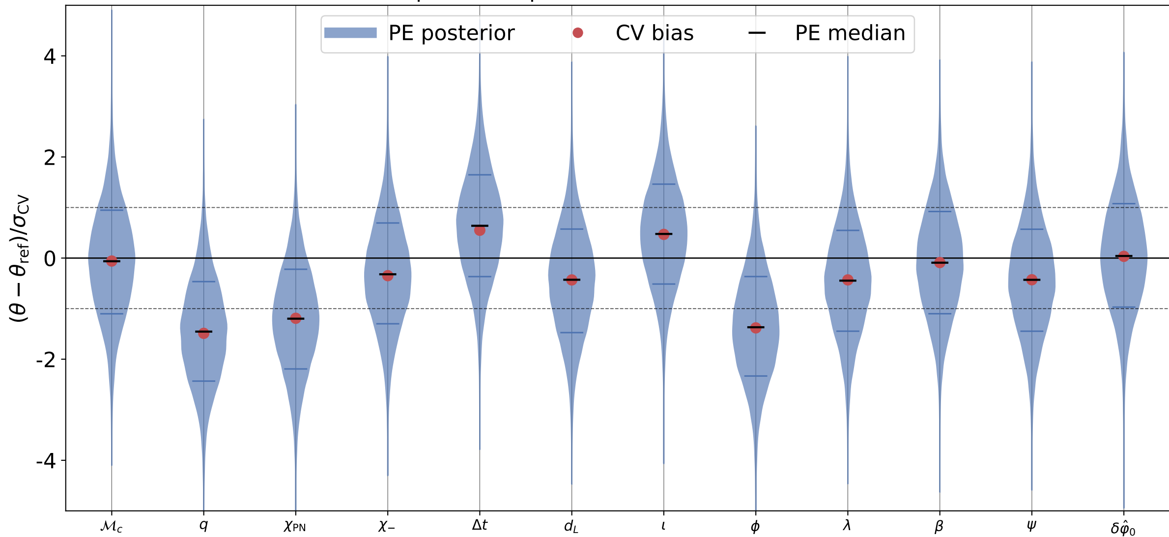
\delta\hat{\phi}_0 recovery, inj_id = 2 processed posterior; reference = truth
