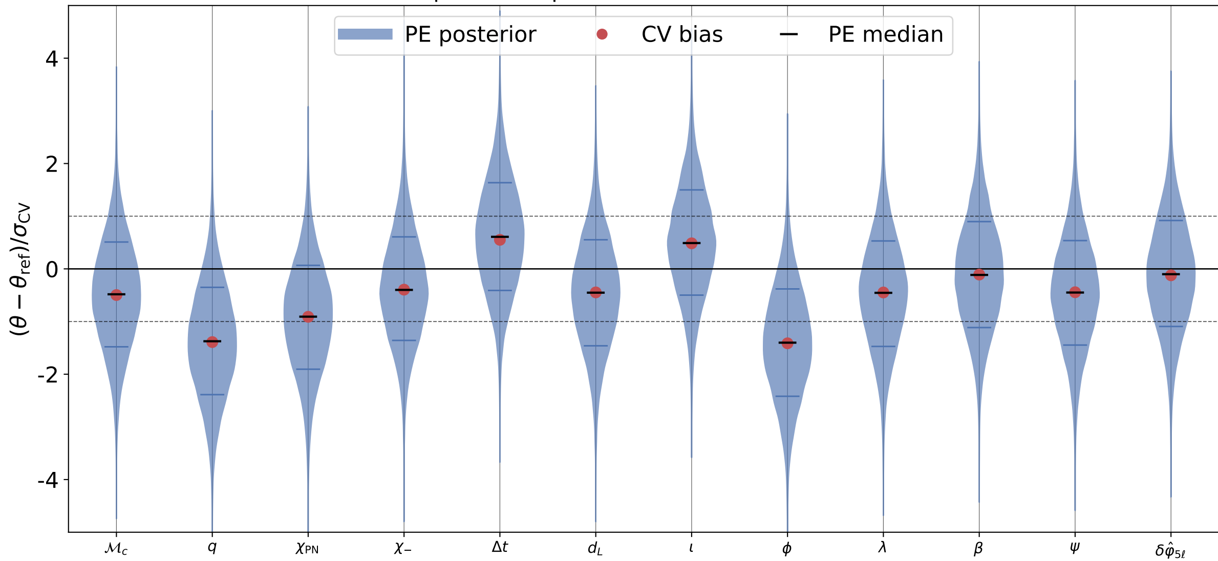
\delta\hat{\phi}_{5\ell} recovery, inj_id = 2 processed posterior; reference = truth
