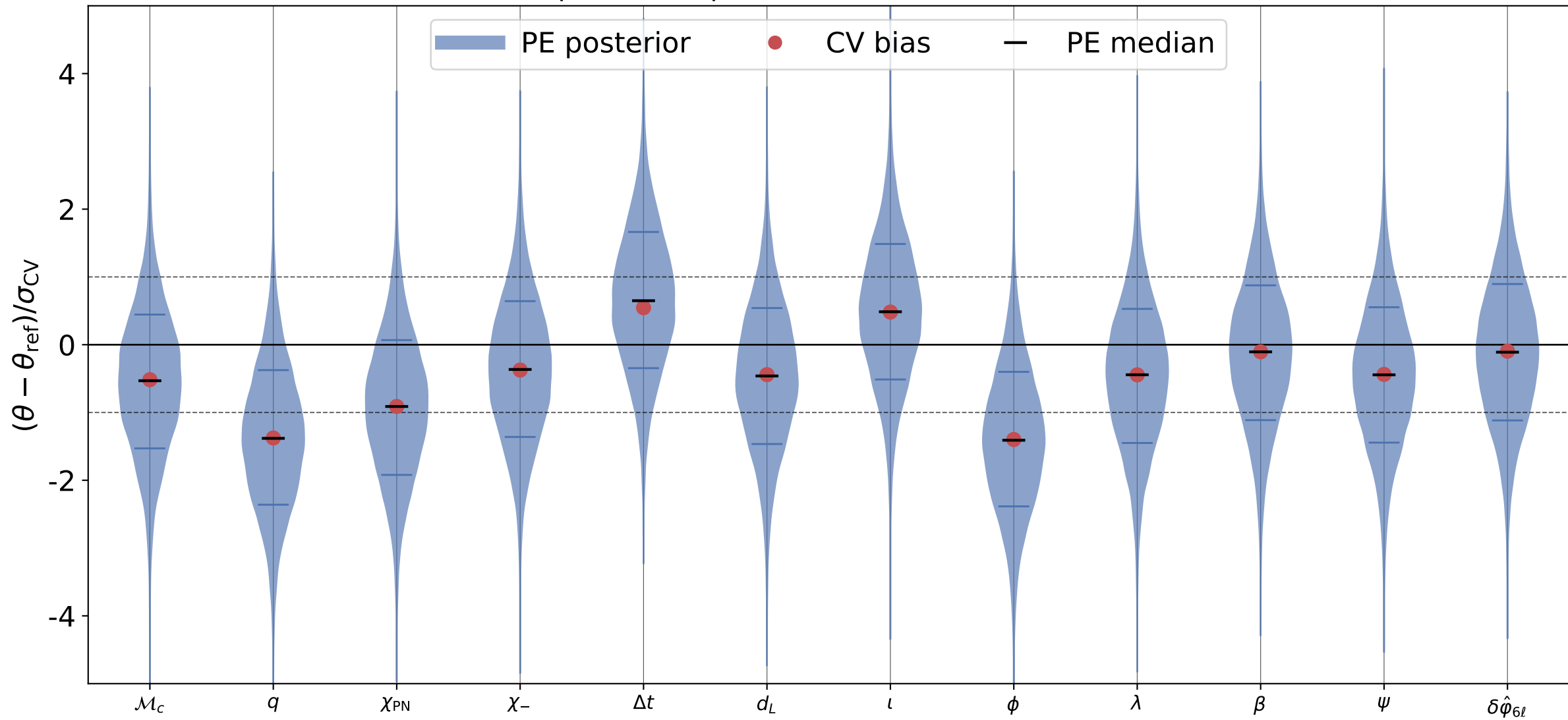
\delta\hat{\phi}_{6\ell} recovery, inj_id = 2 processed posterior; reference = truth
