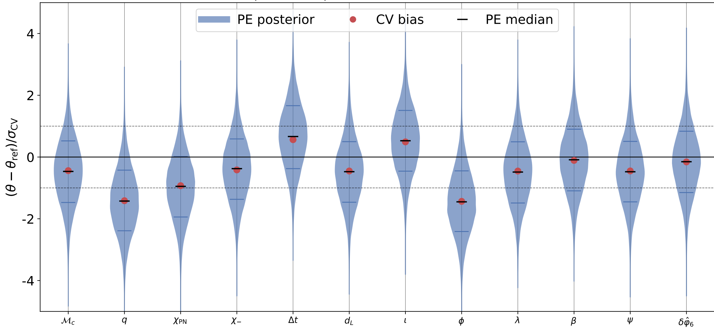
\delta\hat{\phi}_6 recovery, inj_id = 2 processed posterior; reference = truth
