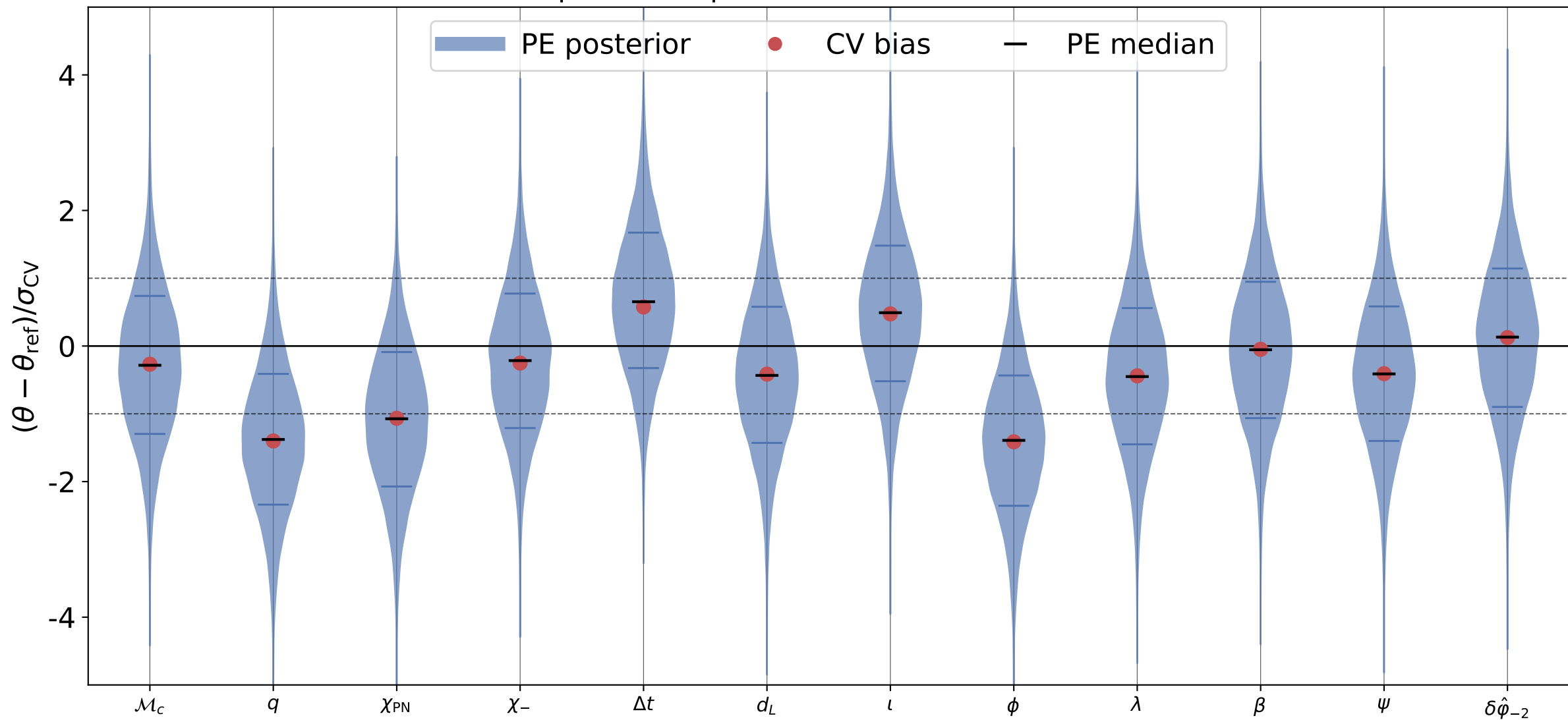
\delta\hat{\phi}_{-2} recovery, inj_id = 2 processed posterior; reference = truth
