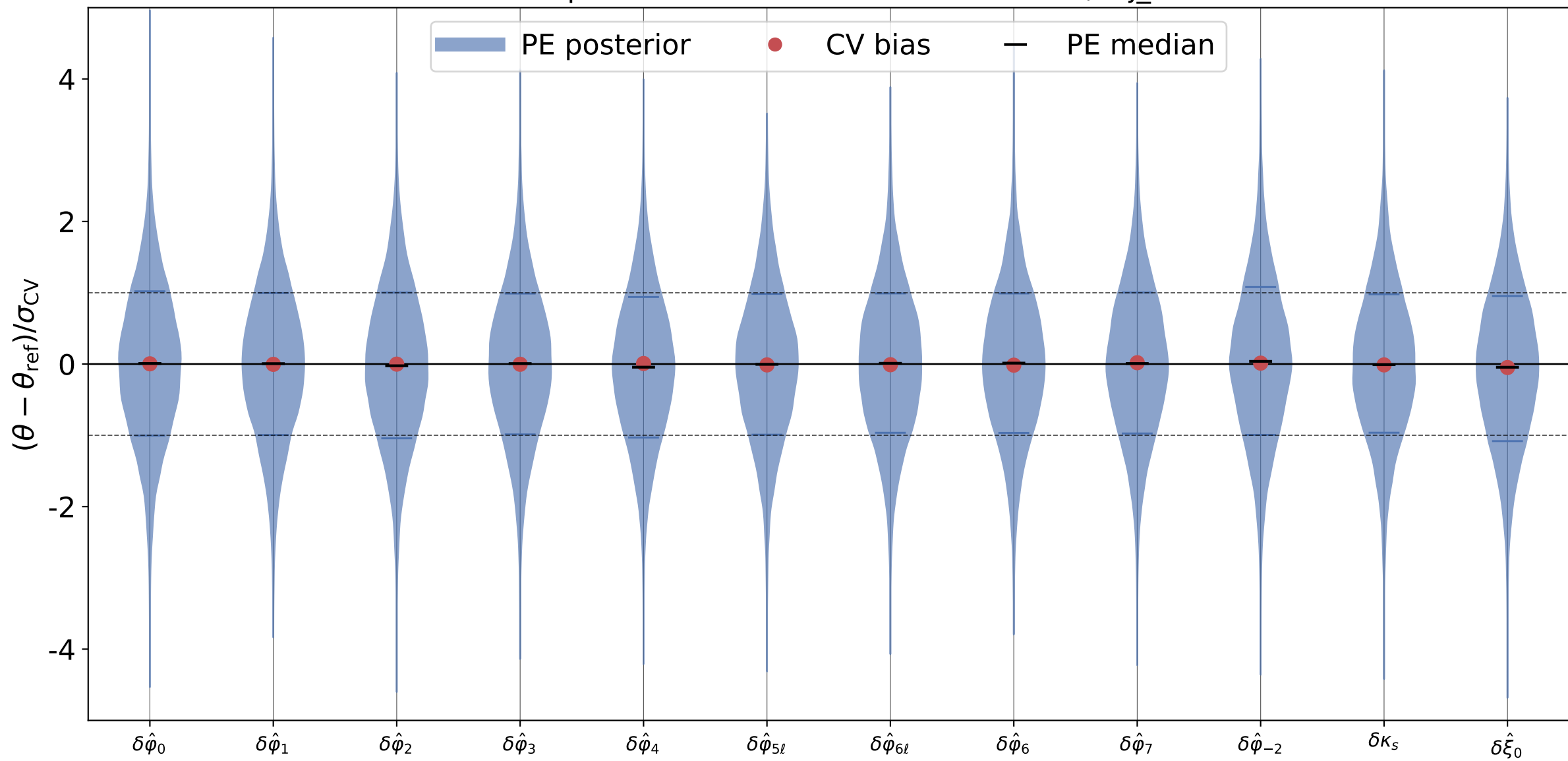
Active FTI posterior distributions and CV biases, inj_id = 3
