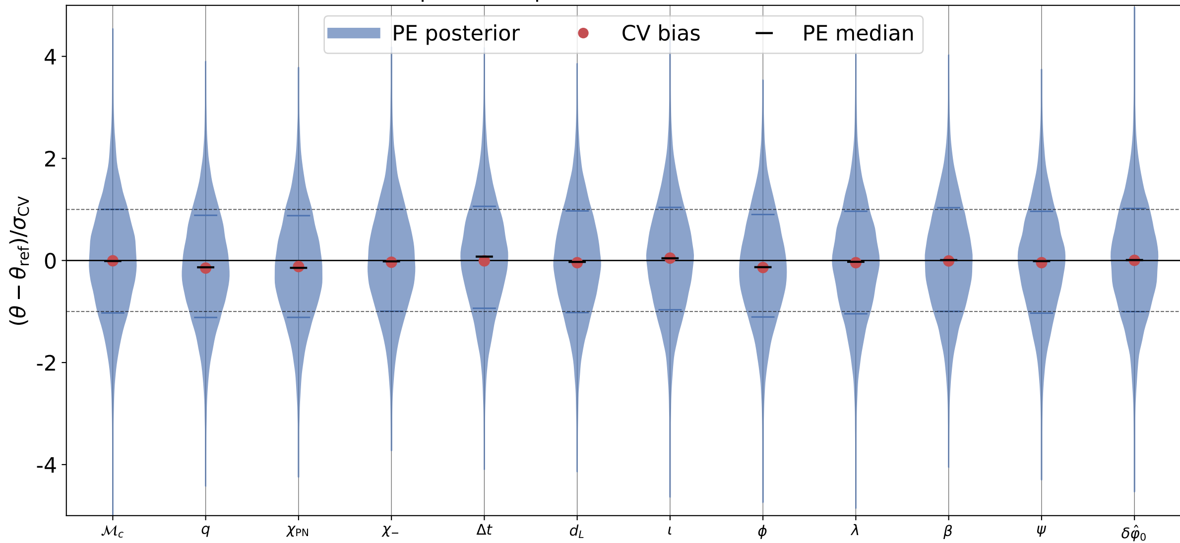
\delta\hat{\phi}_0 recovery, inj_id = 3 processed posterior; reference = truth
