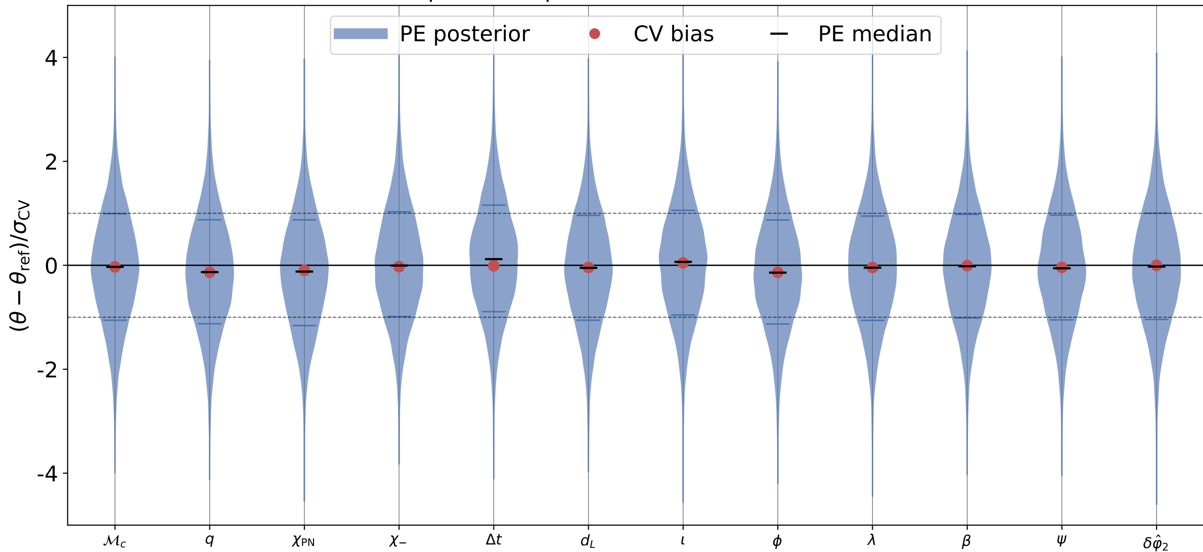
\delta\hat{\phi}_2 recovery, inj_id = 3 processed posterior; reference = truth
