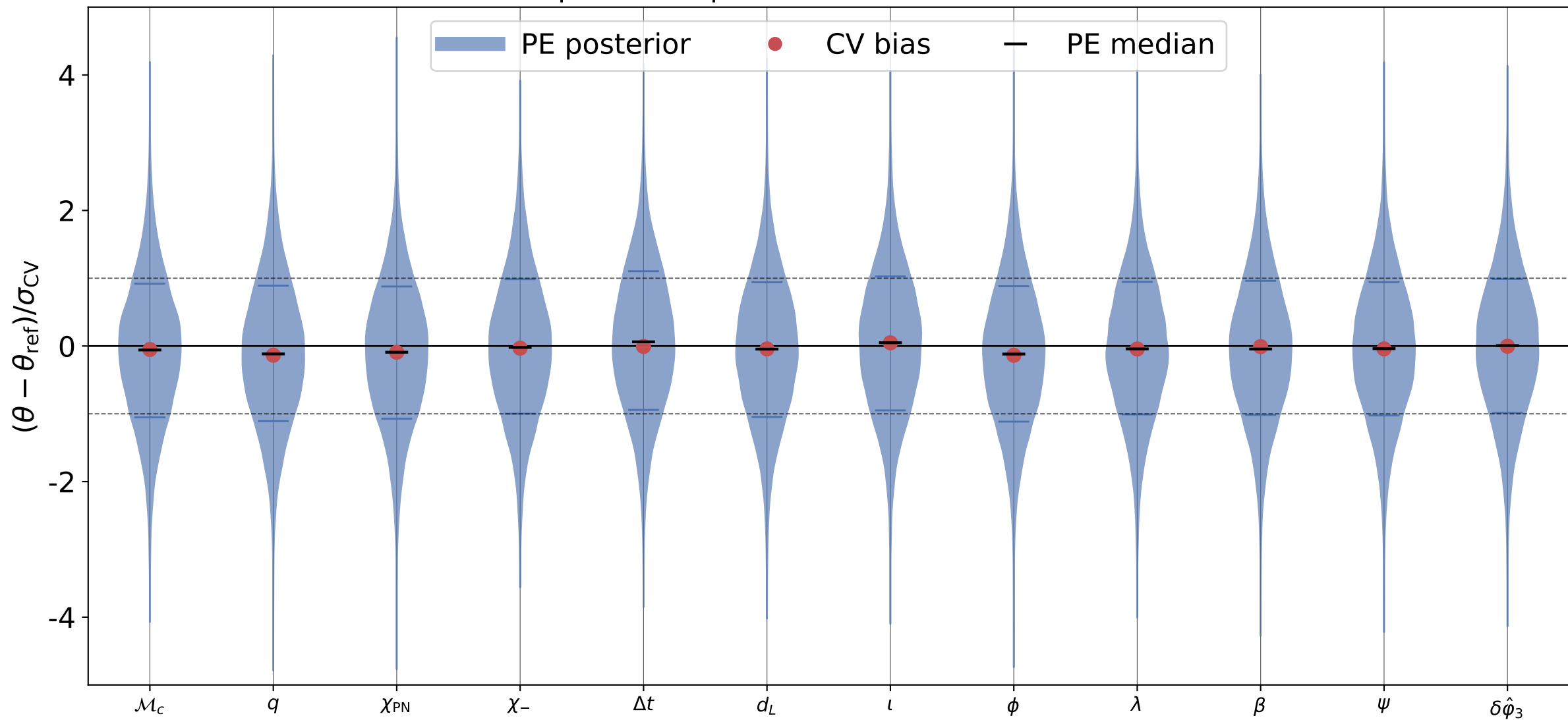
\delta\hat{\phi}_3 recovery, inj_id = 3 processed posterior; reference = truth
