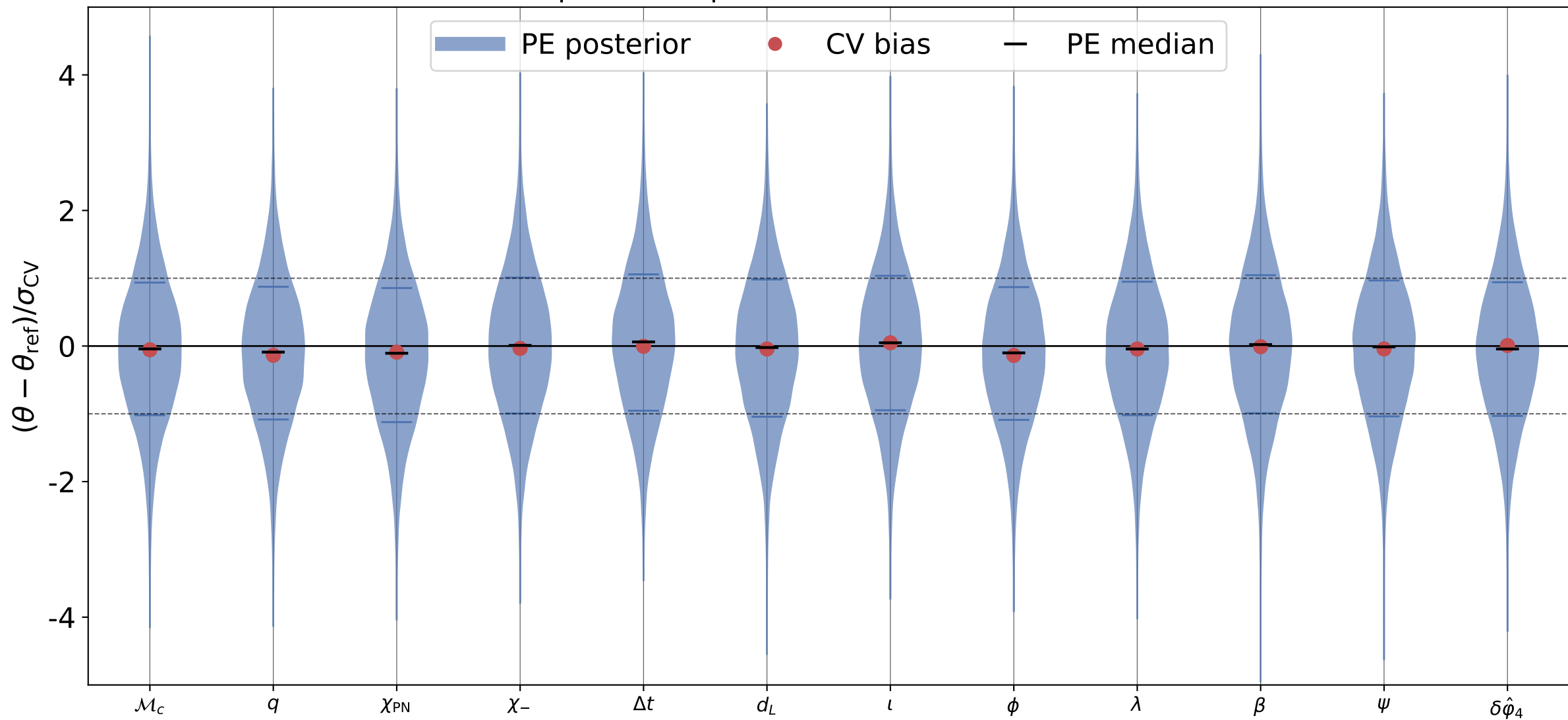
\delta\hat{\phi}_4 recovery, inj_id = 3 processed posterior; reference = truth
