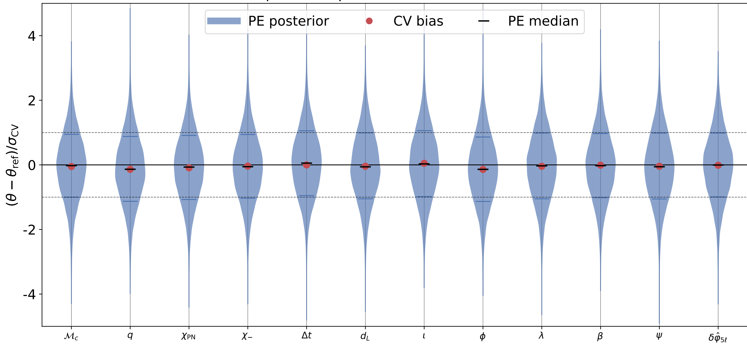
\delta\hat{\phi}_{5\ell} recovery, inj_id = 3 processed posterior; reference = truth
