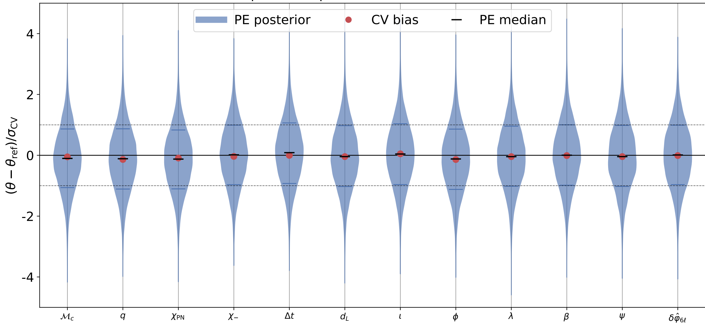
\delta\hat{\phi}_{6\ell} recovery, inj_id = 3 processed posterior; reference = truth
