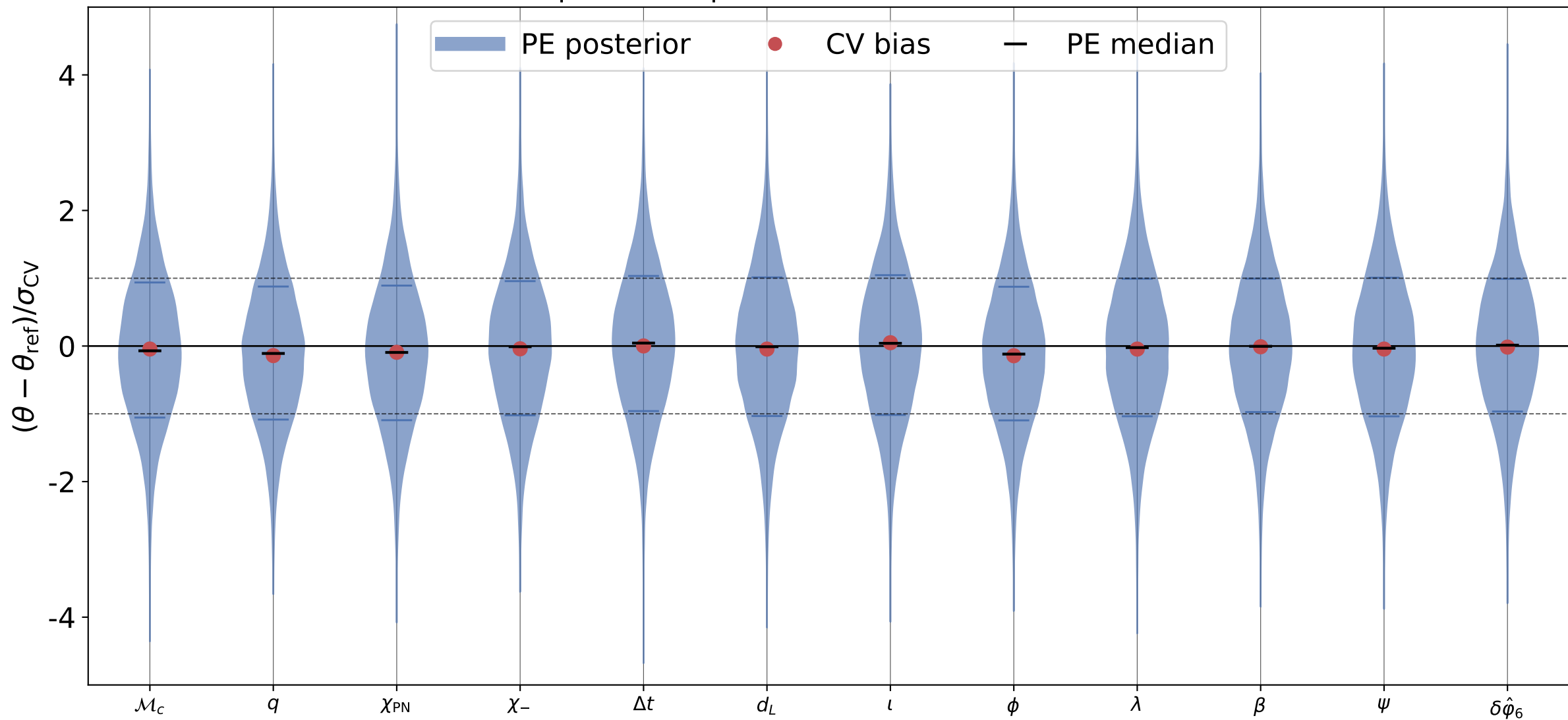
\delta\hat{\phi}_6 recovery, inj_id = 3 processed posterior; reference = truth
