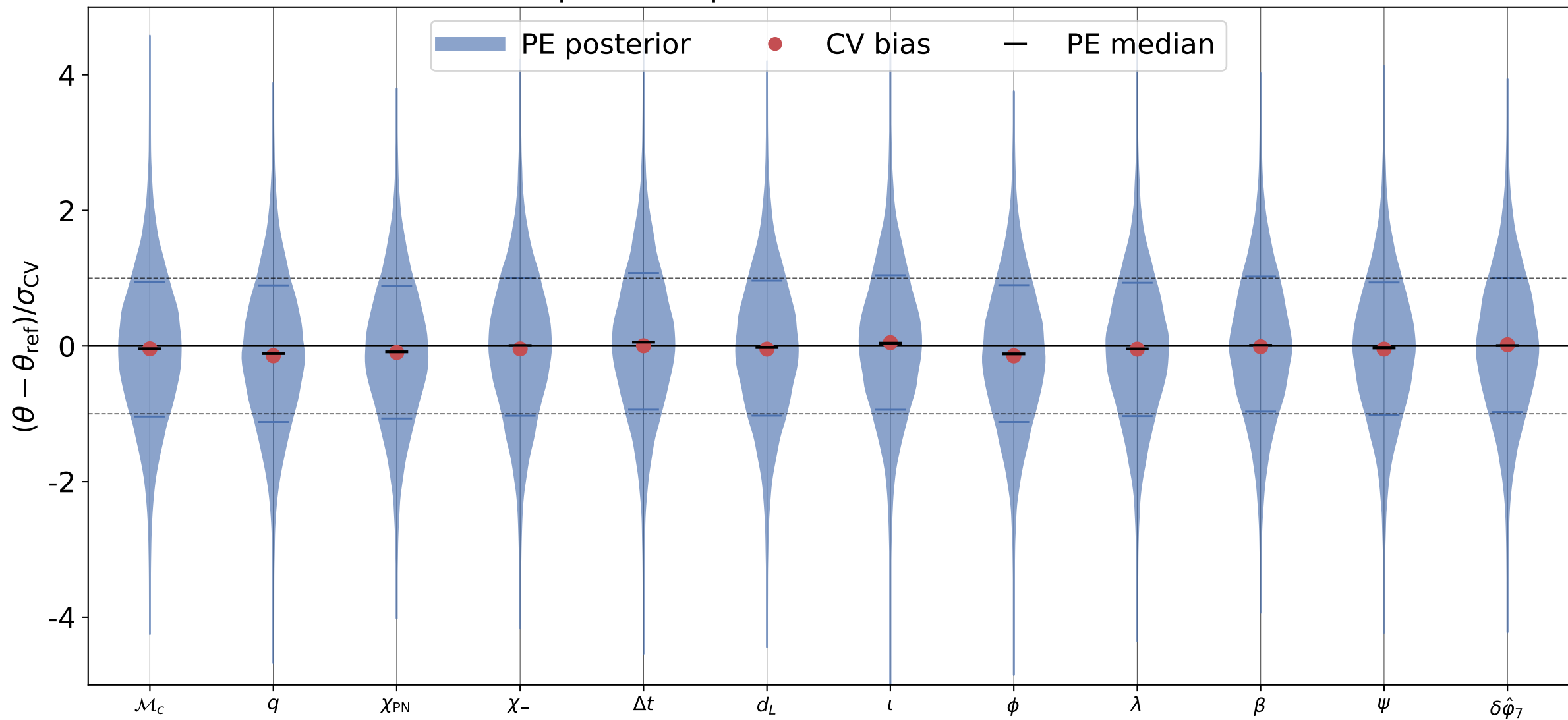
\delta\hat{\phi}_7 recovery, inj_id = 3 processed posterior; reference = truth
