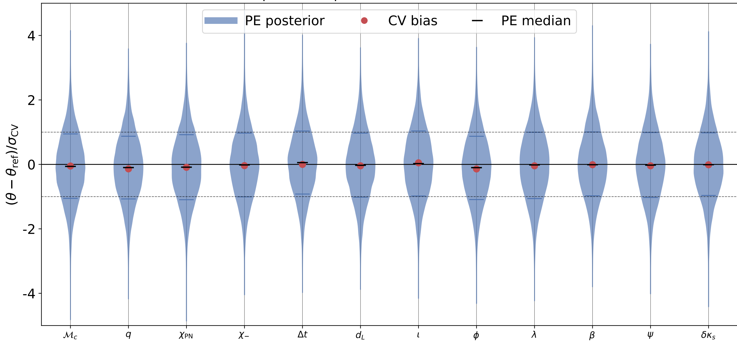
\delta\kappa_s recovery, inj_id = 3 processed posterior; reference = truth
