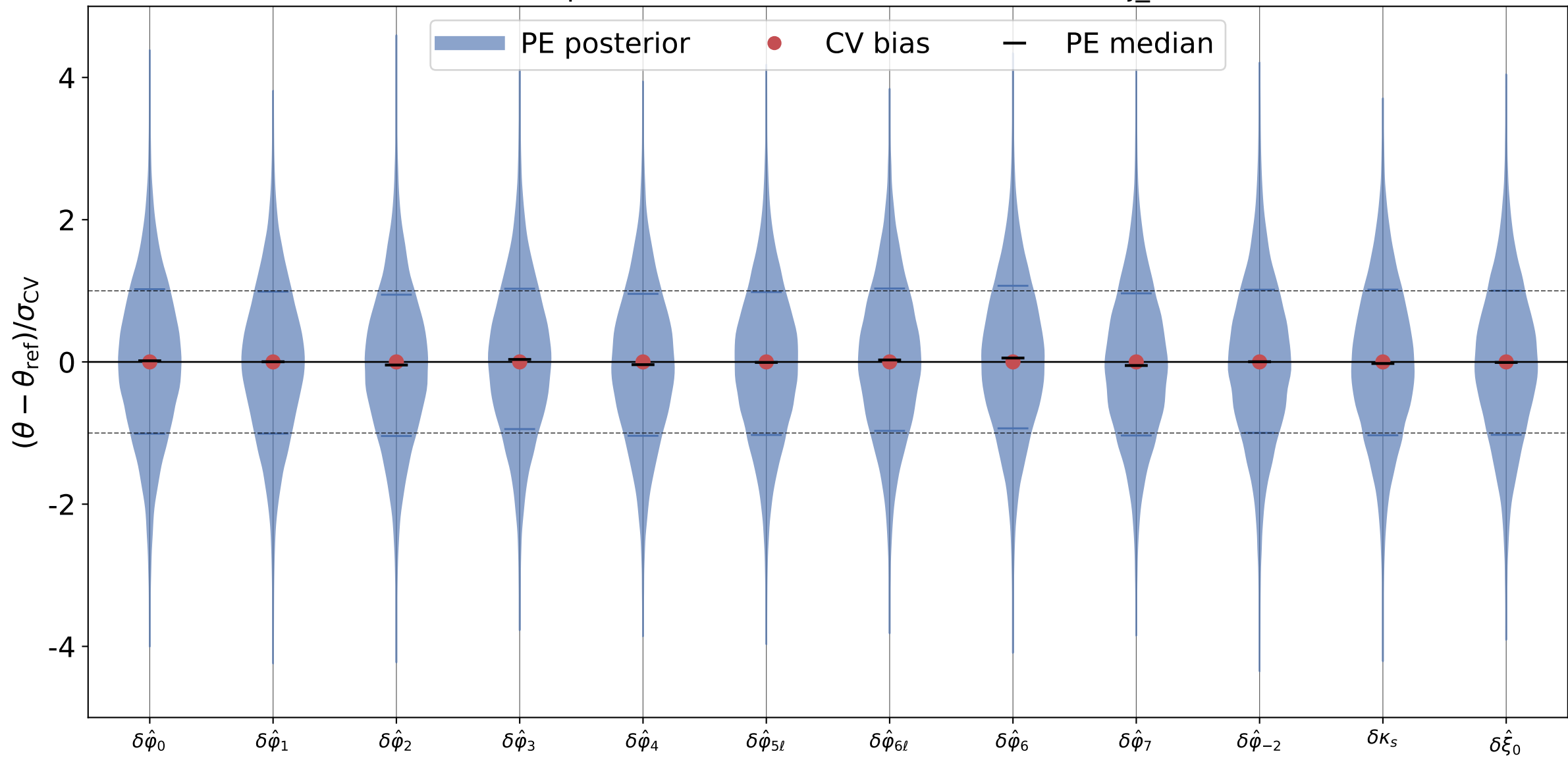
Active FTI posterior distributions and CV biases, inj_id = 4
