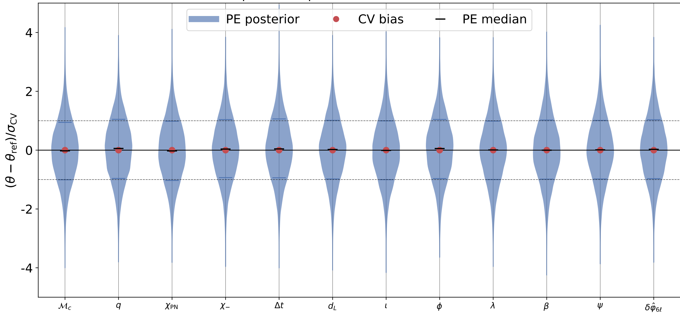
\delta\hat{\phi}_{6\ell} recovery, inj_id = 4 processed posterior; reference = truth
