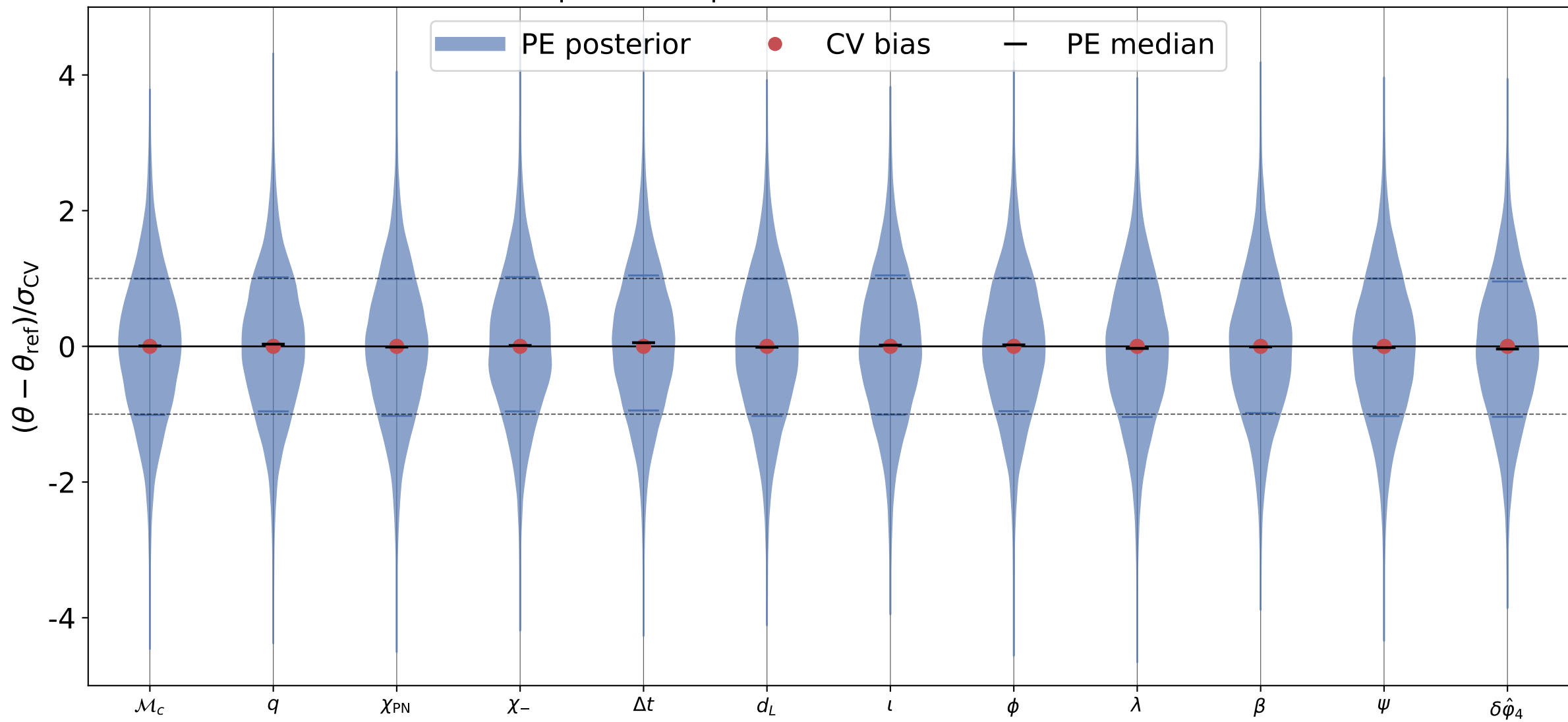
\delta\hat{\phi}_4 recovery, inj_id = 4 processed posterior; reference = truth
