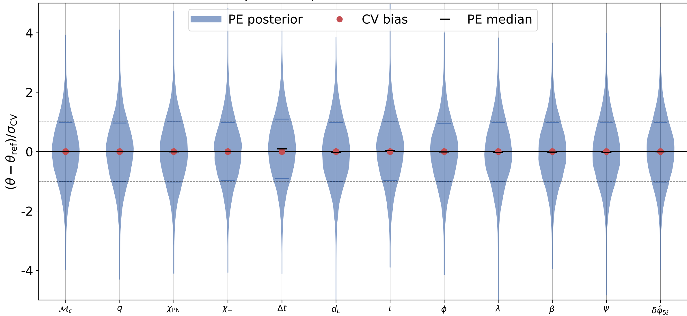
\delta\hat{\phi}_{5\ell} recovery, inj_id = 4 processed posterior; reference = truth
