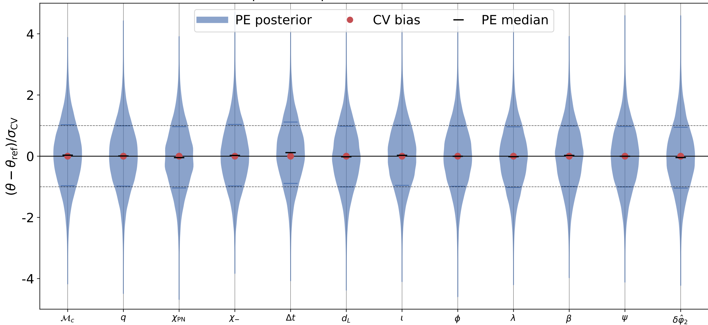
\delta\hat{\phi}_2 recovery, inj_id = 4 processed posterior; reference = truth
