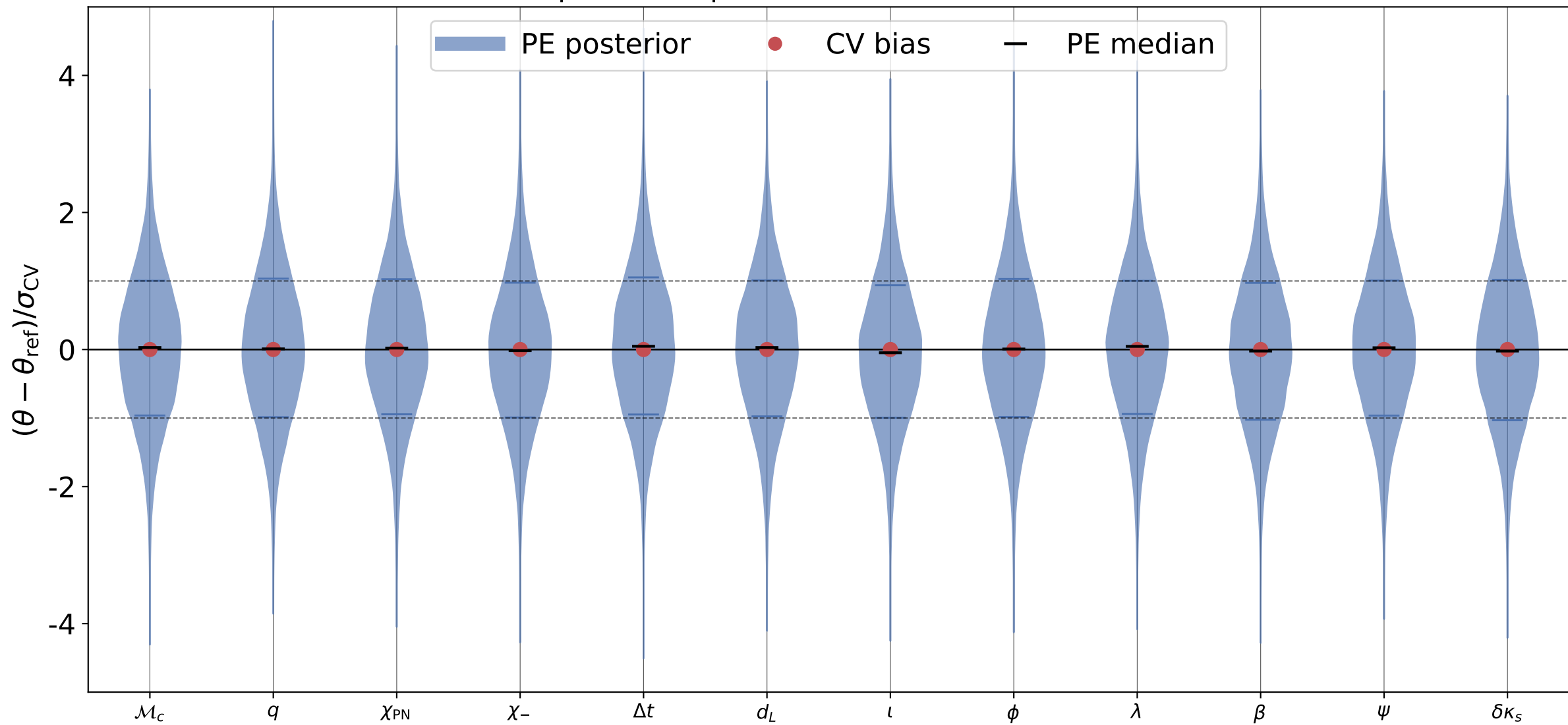
\delta\kappa_s recovery, inj_id = 4 processed posterior; reference = truth
