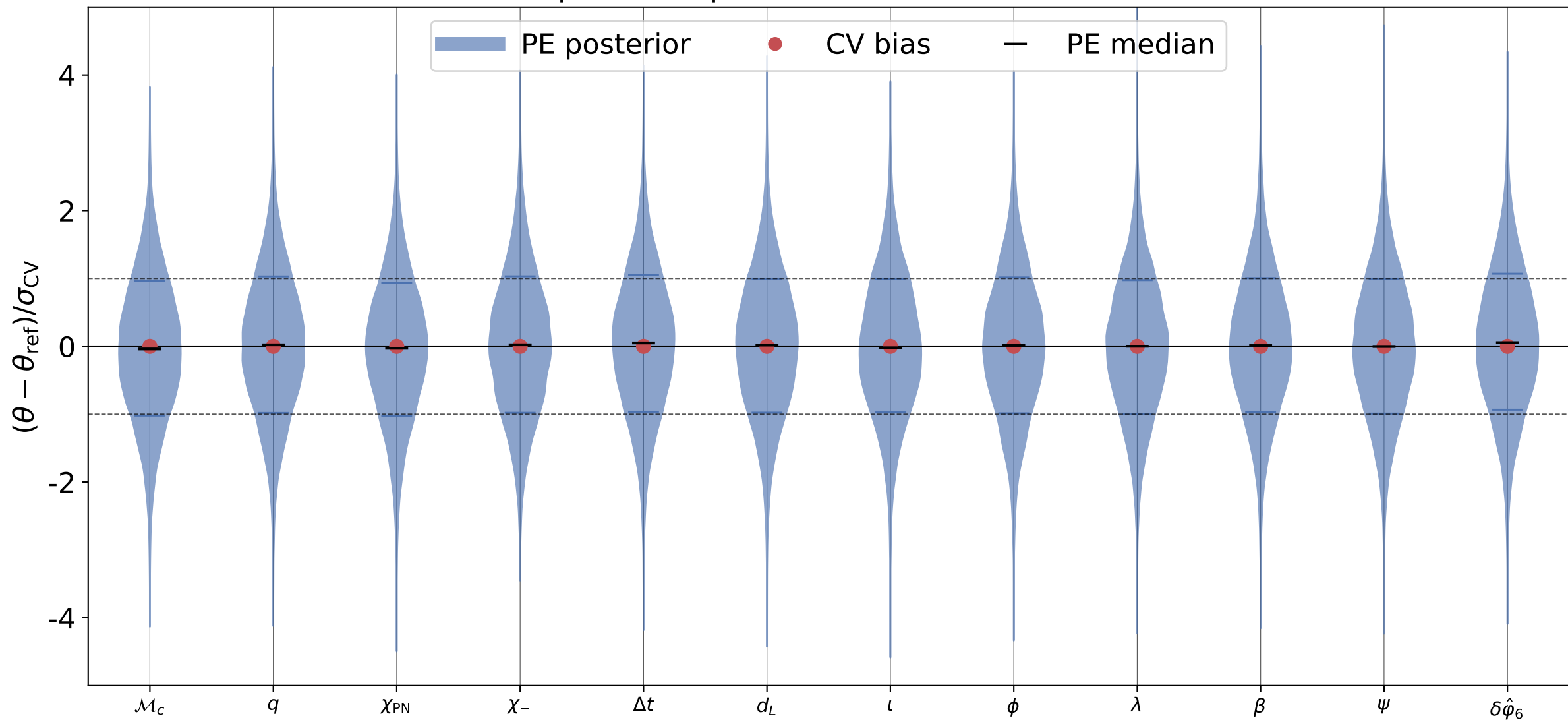
\delta\hat{\phi}_6 recovery, inj_id = 4 processed posterior; reference = truth
