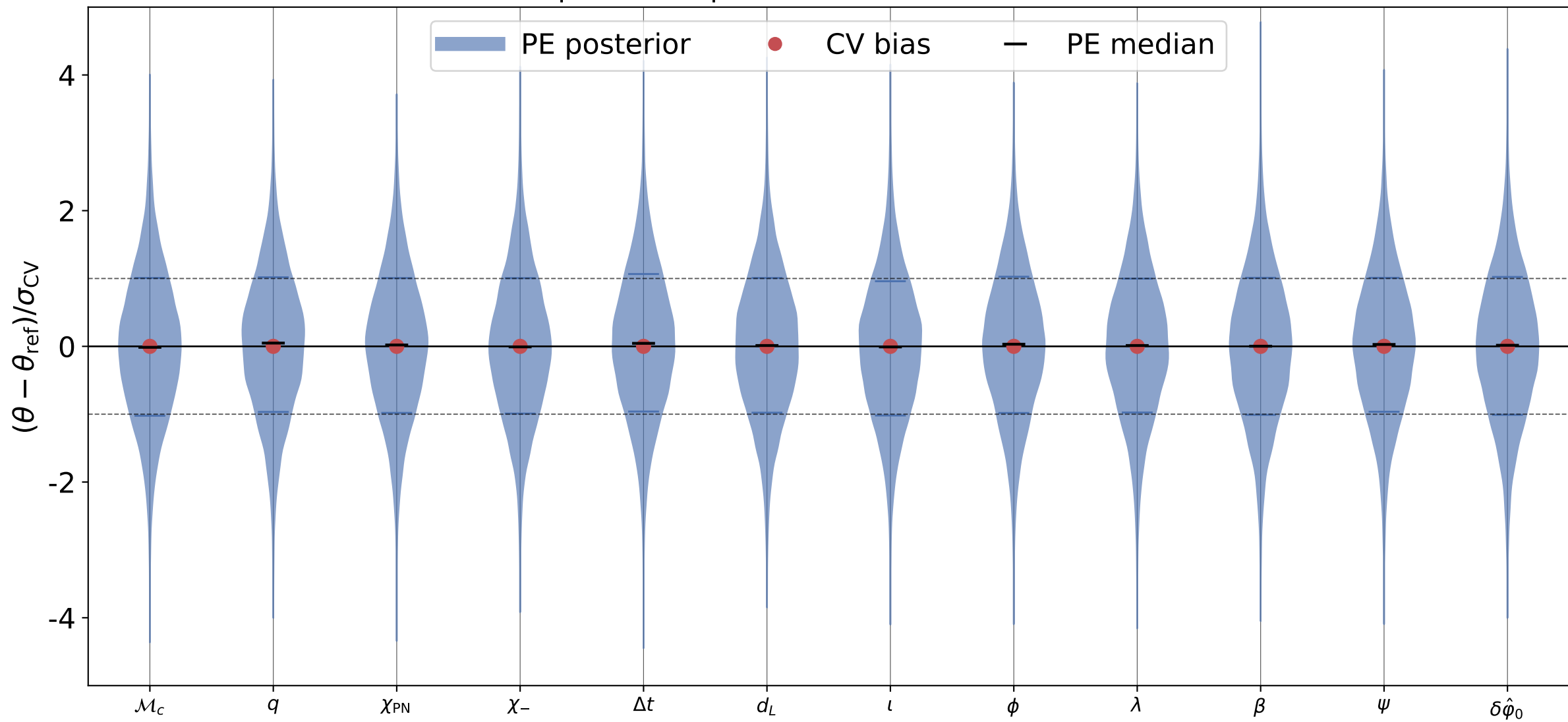
\delta\hat{\phi}_0 recovery, inj_id = 4 processed posterior; reference = truth
