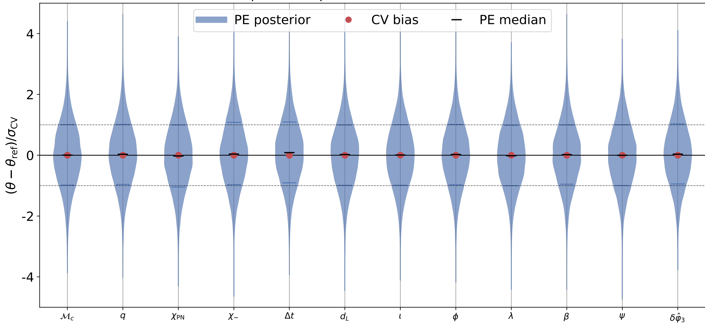
\delta\hat{\phi}_3 recovery, inj_id = 4 processed posterior; reference = truth
