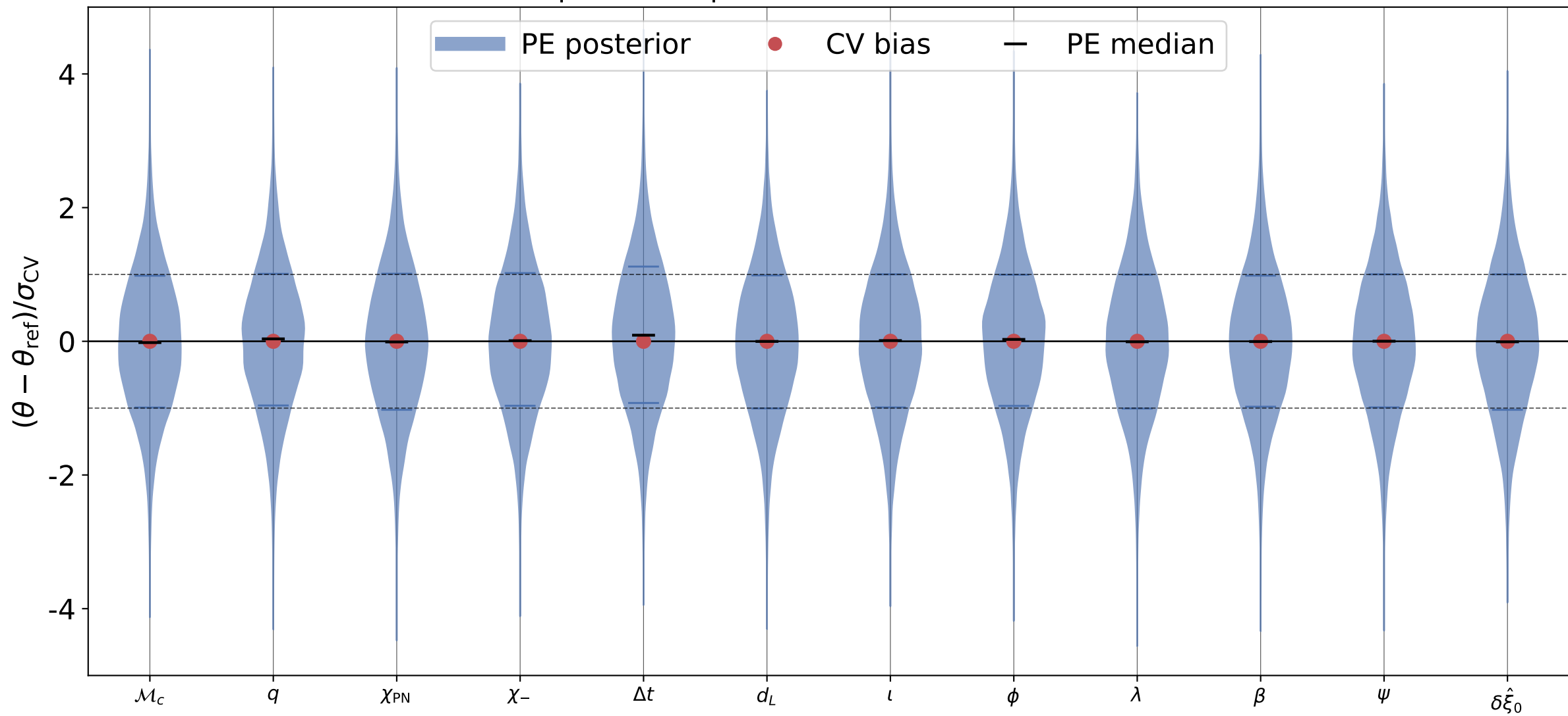
\hat{\delta\xi_0} recovery, inj_id = 4 processed posterior; reference = truth
