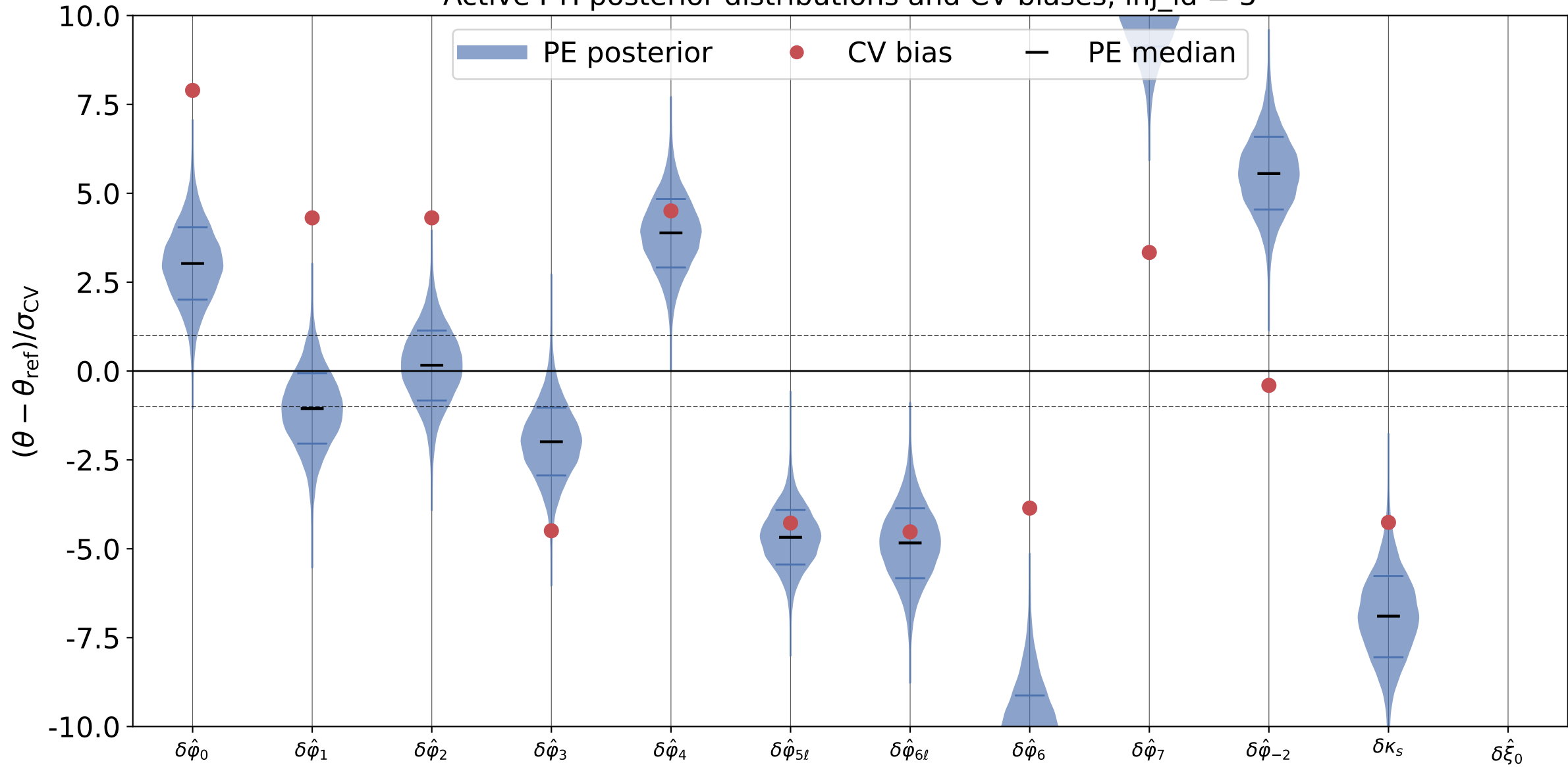
Active FTI posterior distributions and CV biases, inj_id = 5
