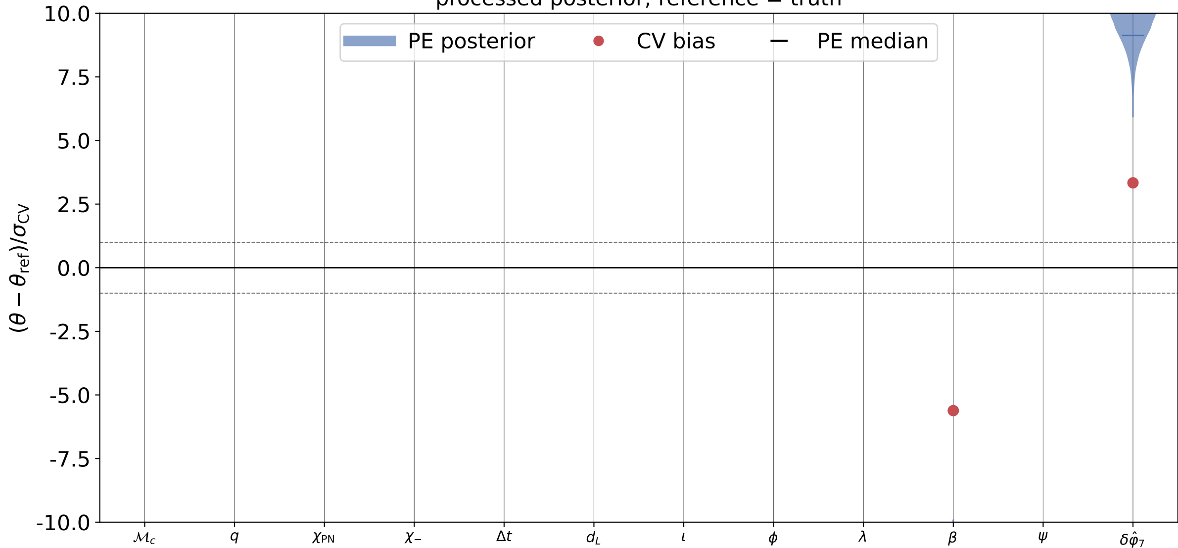
\delta\hat{\phi}_7 recovery, inj_id = 5 processed posterior; reference = truth
