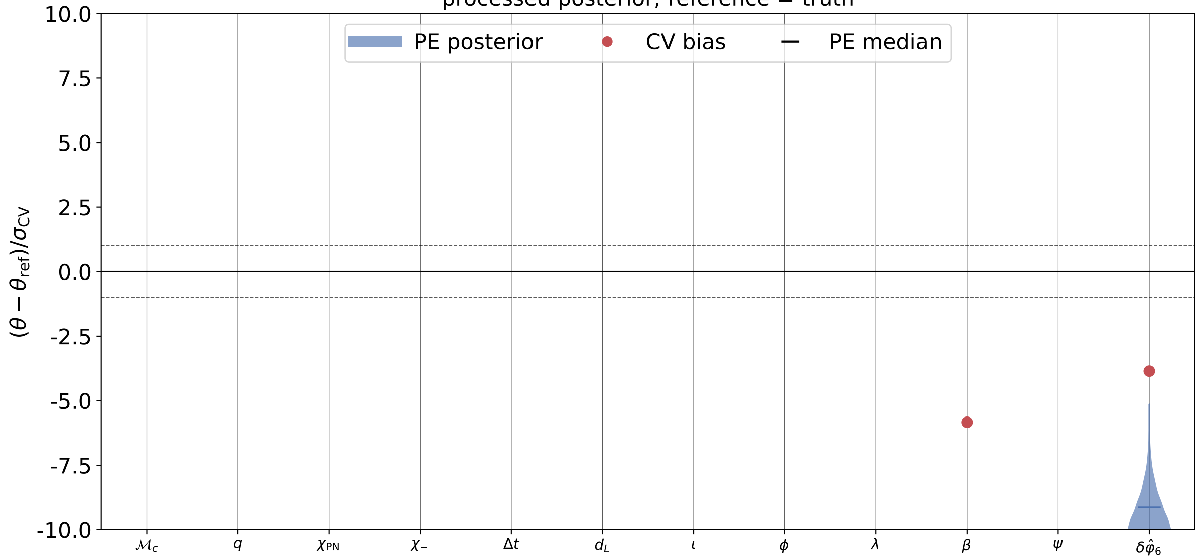
\delta\hat{\phi}_6 recovery, inj_id = 5 processed posterior; reference = truth
