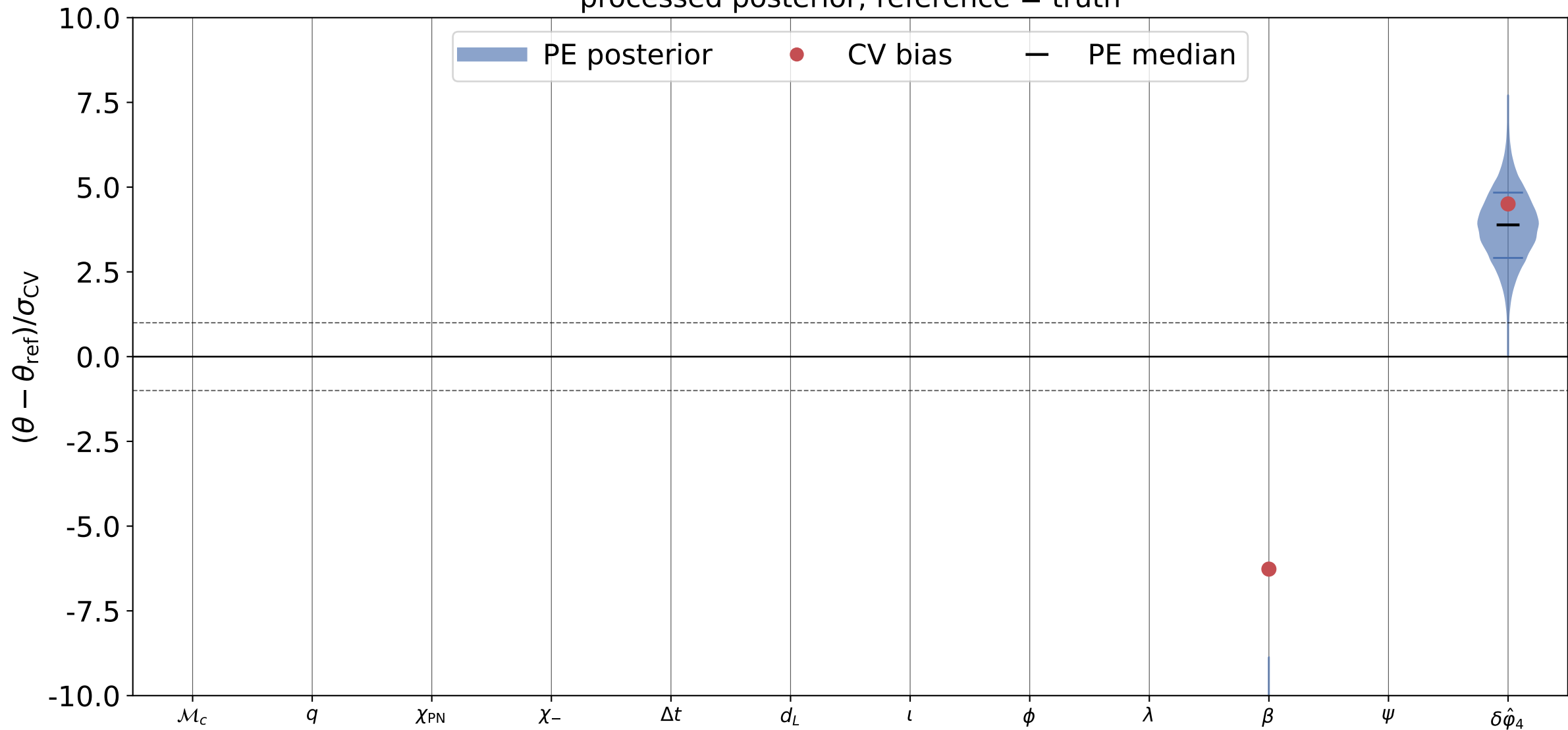
\delta\hat{\phi}_4 recovery, inj_id = 5 processed posterior; reference = truth
