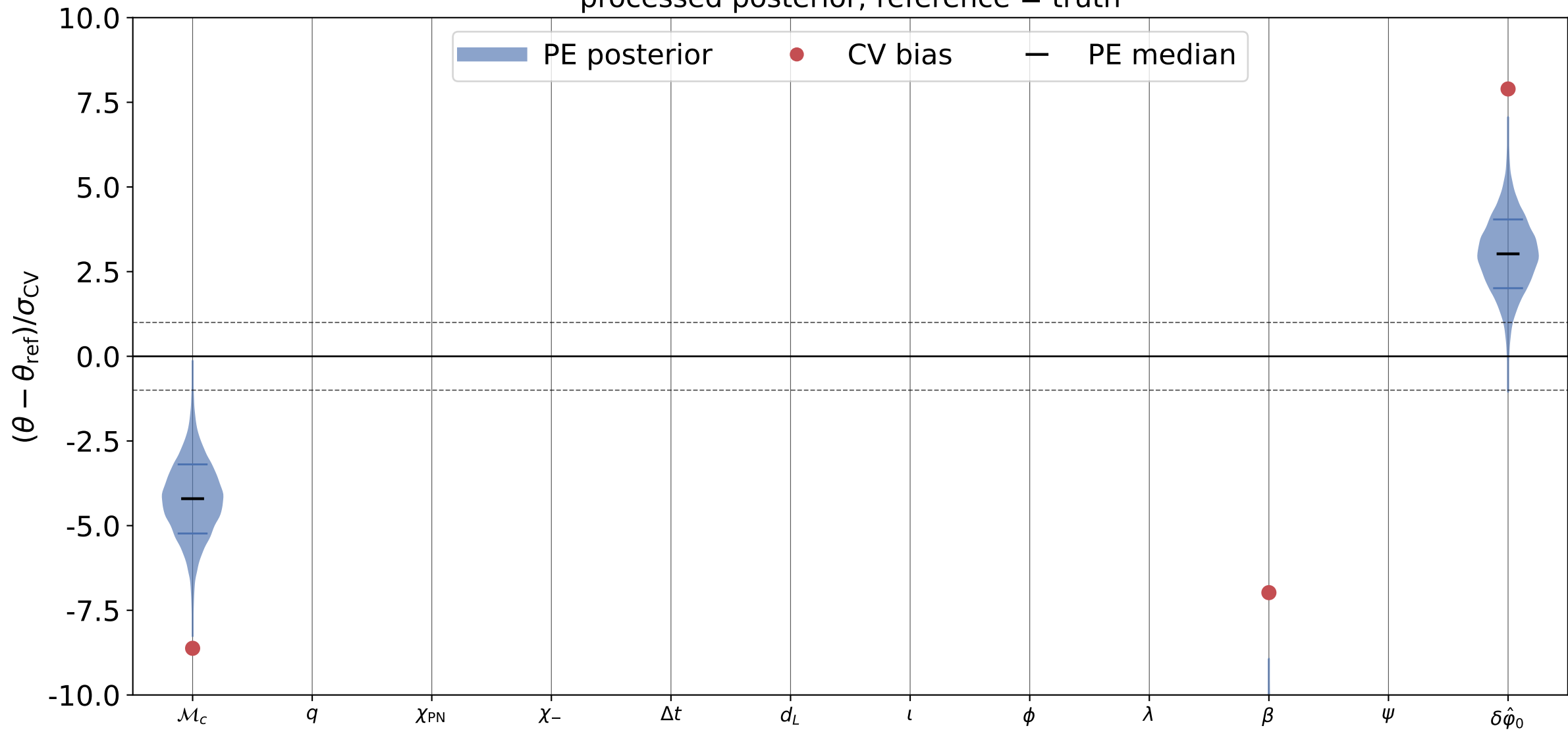
\delta\hat{\phi}_0 recovery, inj_id = 5 processed posterior; reference = truth
