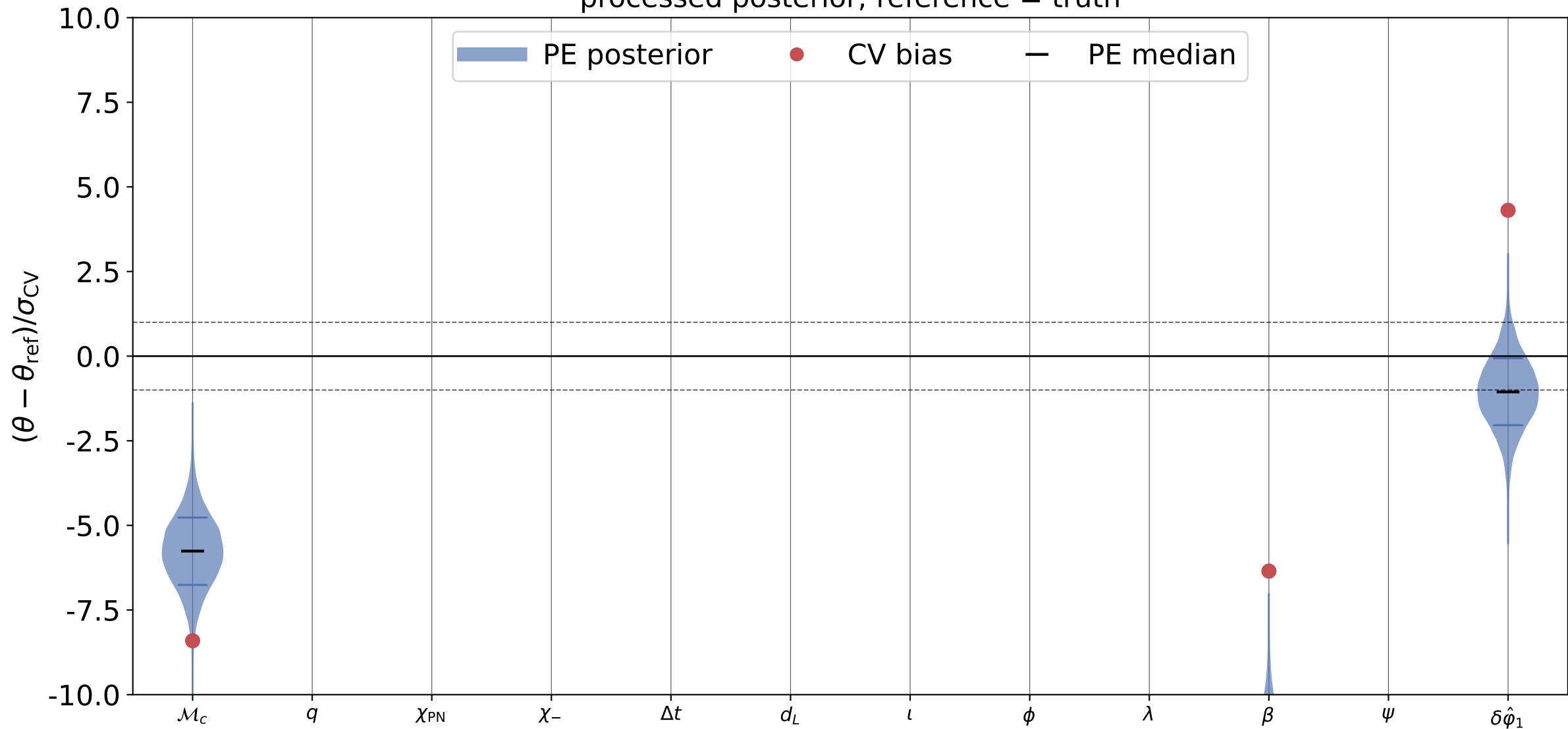
\delta\hat{\phi}_1 recovery, inj_id = 5 processed posterior; reference = truth
