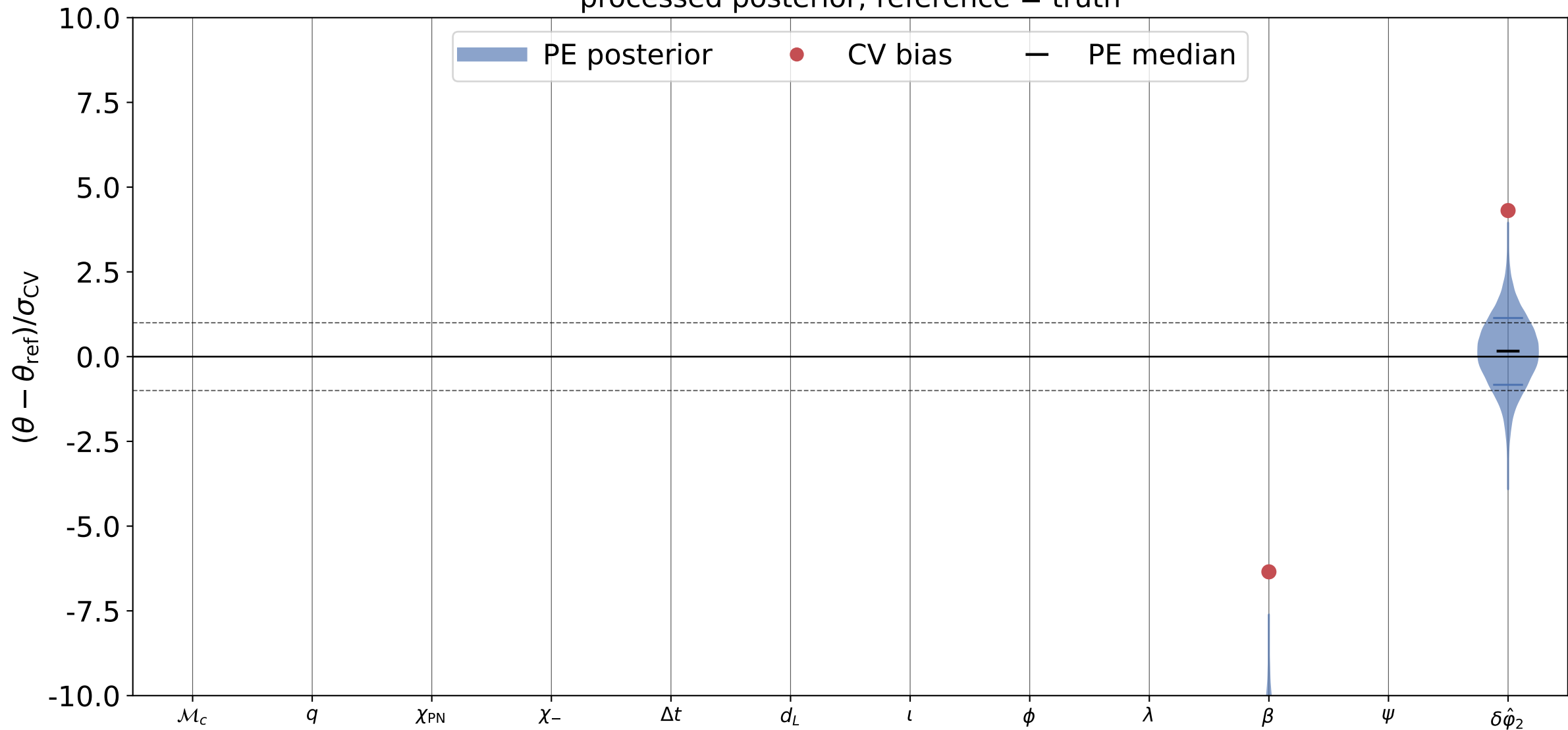
\delta\hat{\phi}_2 recovery, inj_id = 5 processed posterior; reference = truth
