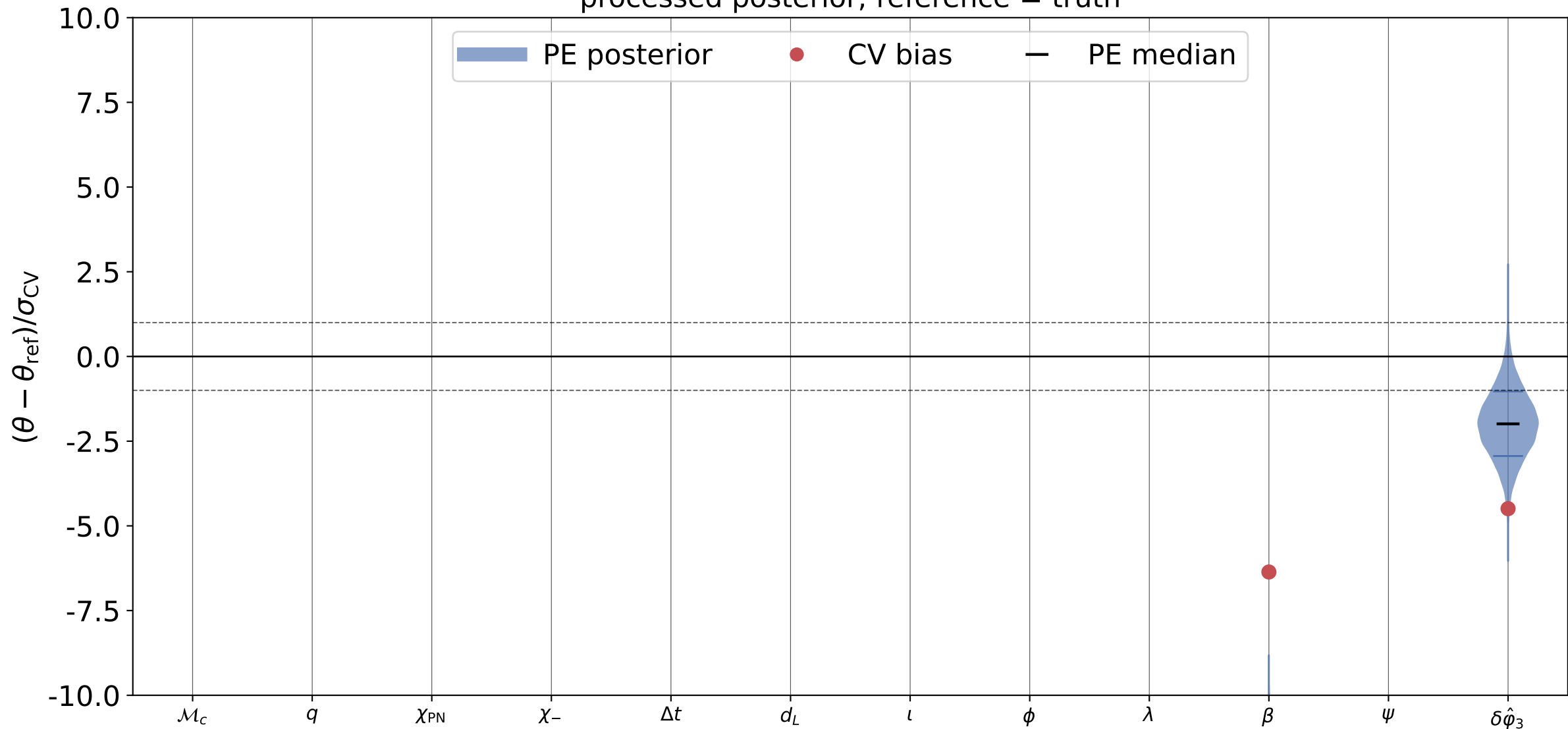
\delta\hat{\phi}_3 recovery, inj_id = 5 processed posterior; reference = truth
