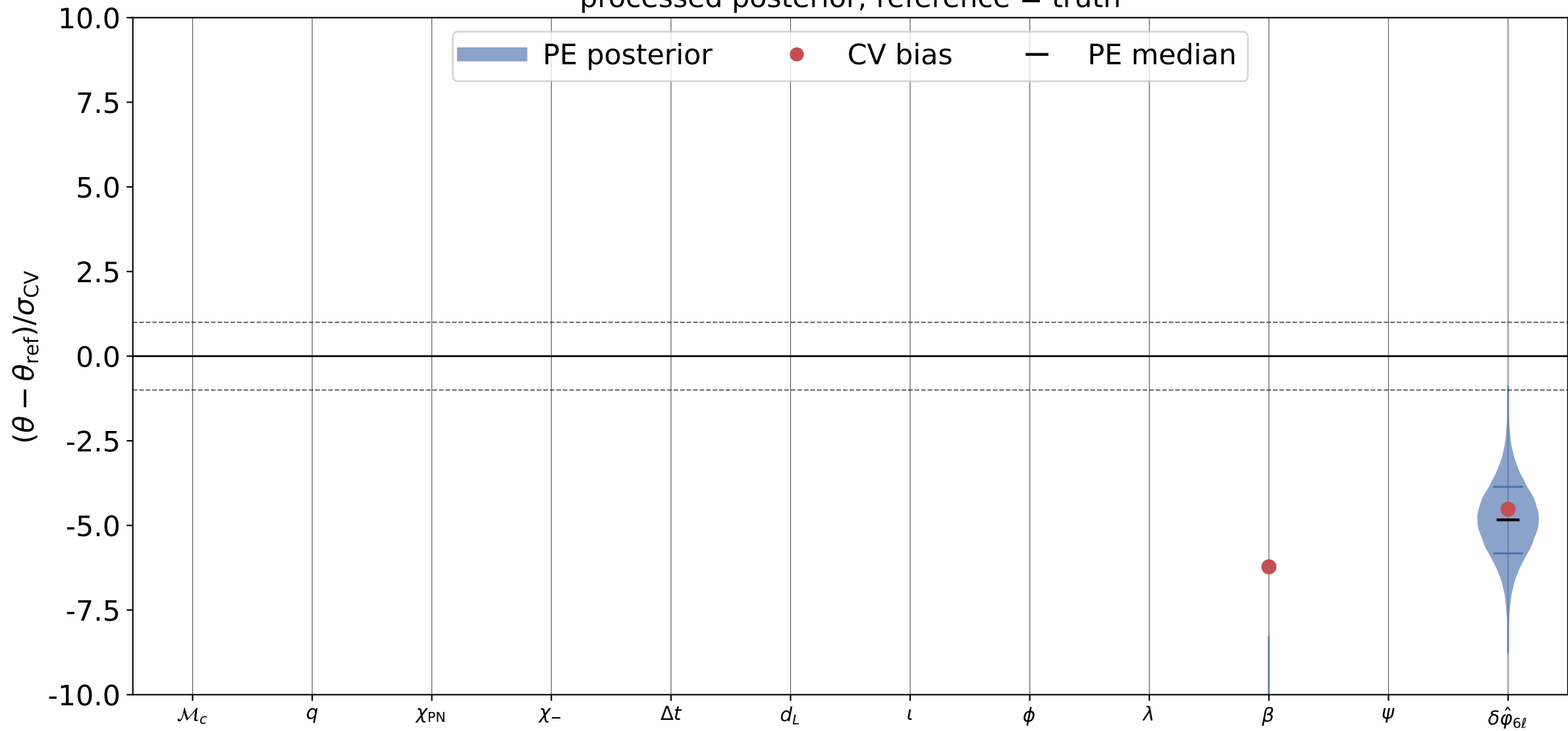
\delta\hat{\phi}_{6\ell} recovery, inj_id = 5 processed posterior; reference = truth
