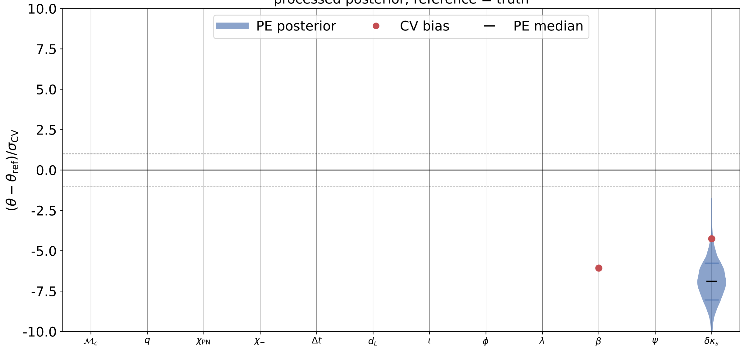
\delta\kappa_s recovery, inj_id = 5 processed posterior; reference = truth
