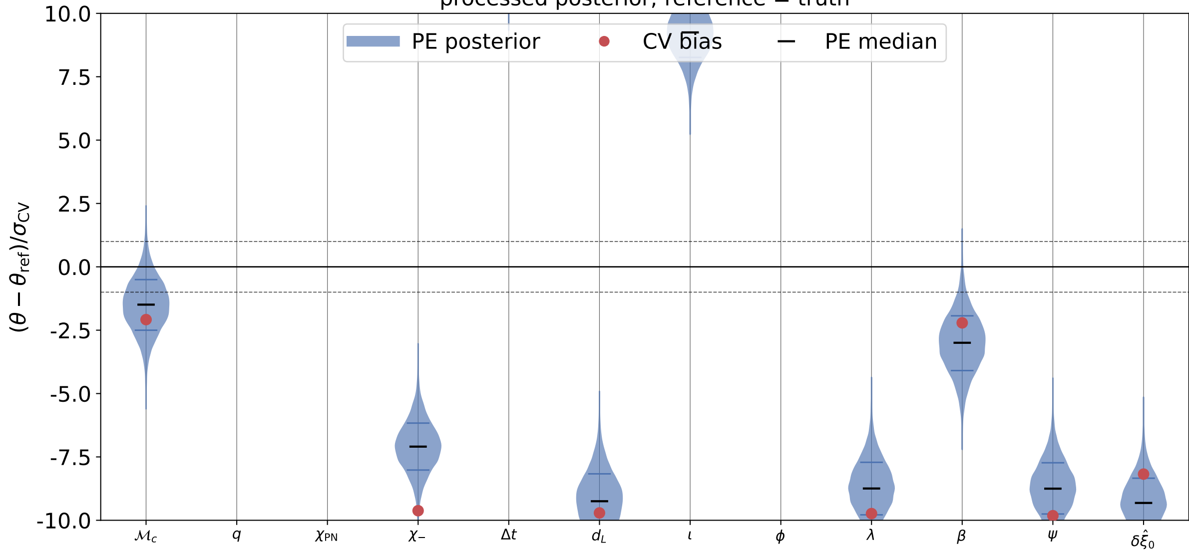
\hat{\delta\xi_0} recovery, inj_id = 6 processed posterior; reference = truth
