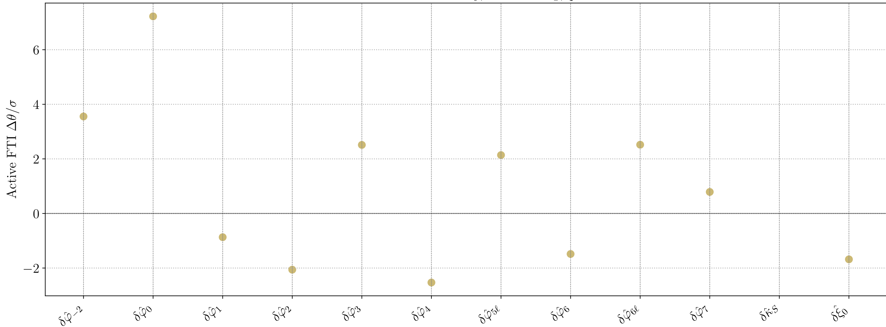
Active-FTI bias summary, M = 10^6 M_\odot , q = 1
