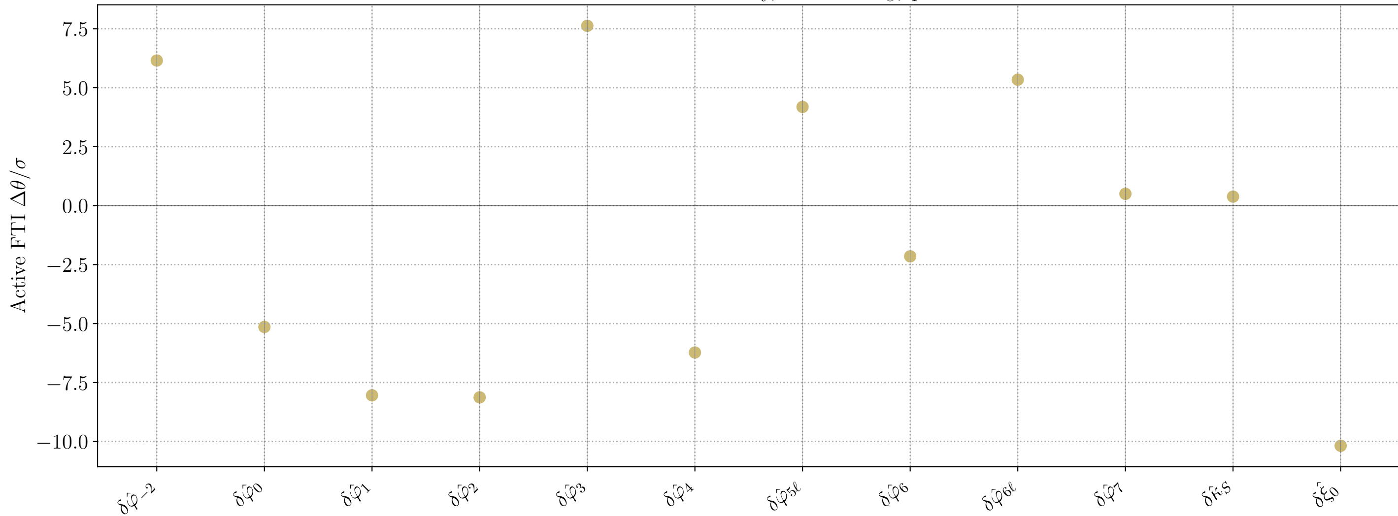
Active-FTI bias summary, M = 10^6 M_\odot , q = 2
