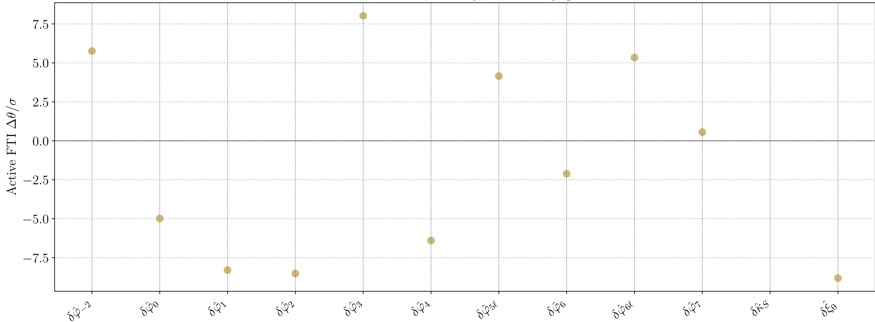
Active-FTI bias summary, M = 10^6 M_\odot , q = 3
