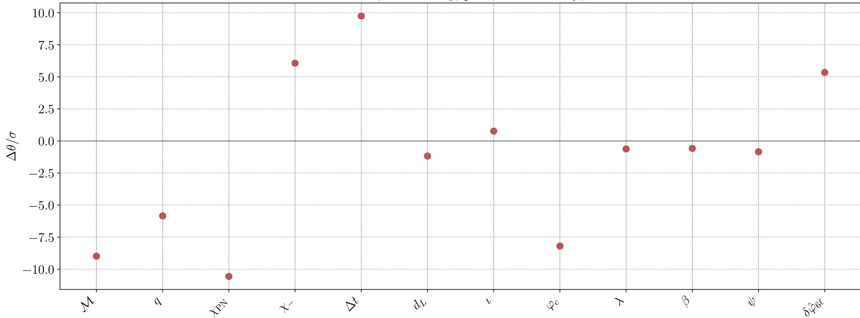
CV bias, M = 10^6 M_\odot , q = 3 , active FTI: \delta\hat{\varphi}_{6\ell}
