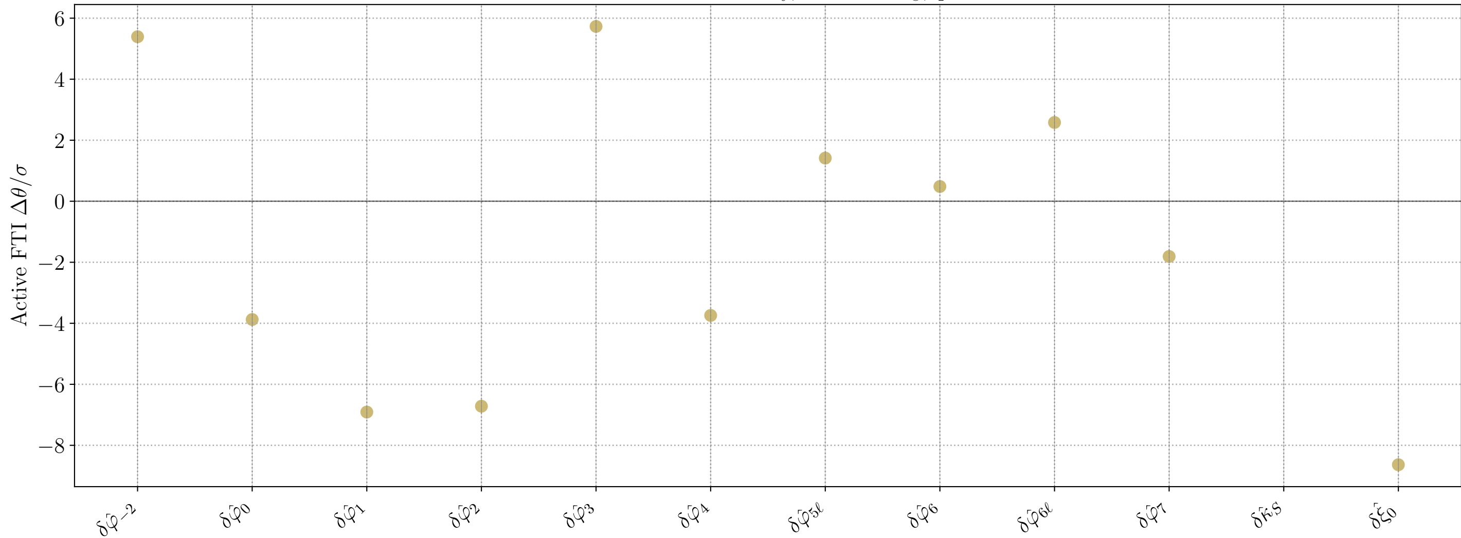
Active-FTI bias summary, M = 10^6 M_\odot , q = 4
