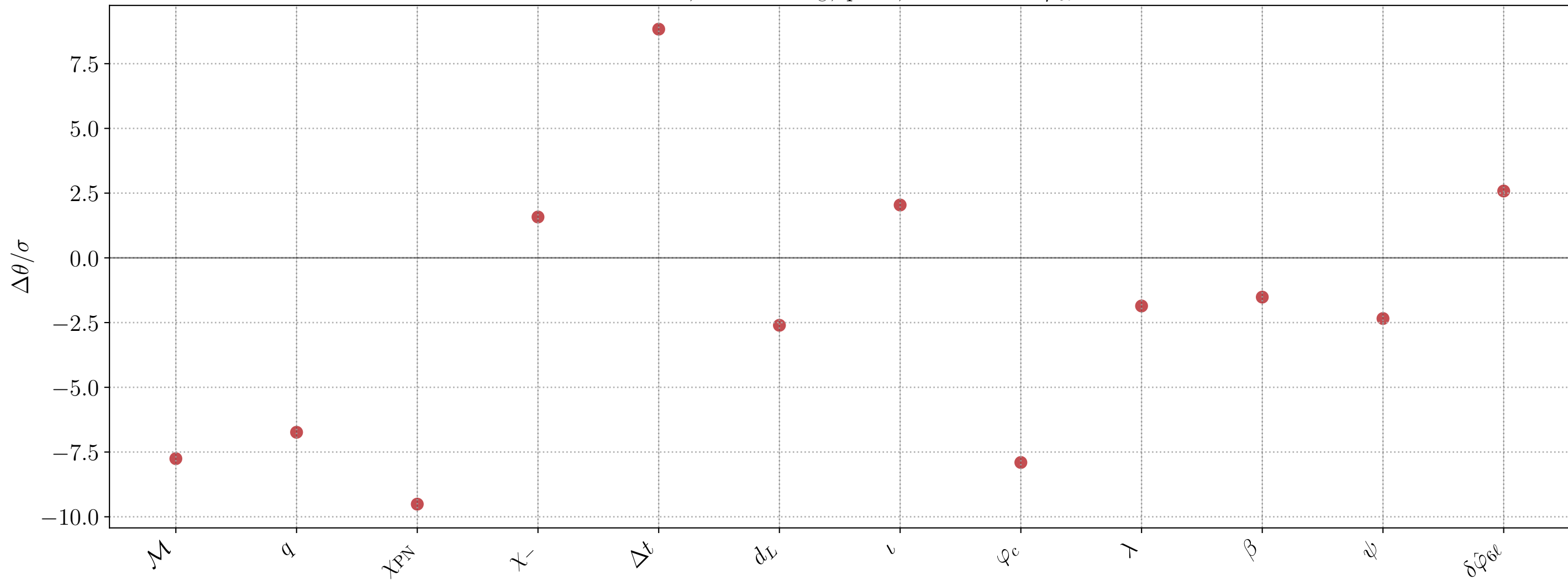
CV bias, M = 10^6 M_\odot , q = 4 , active FTI: \delta\hat{\varphi}_{6\ell}
