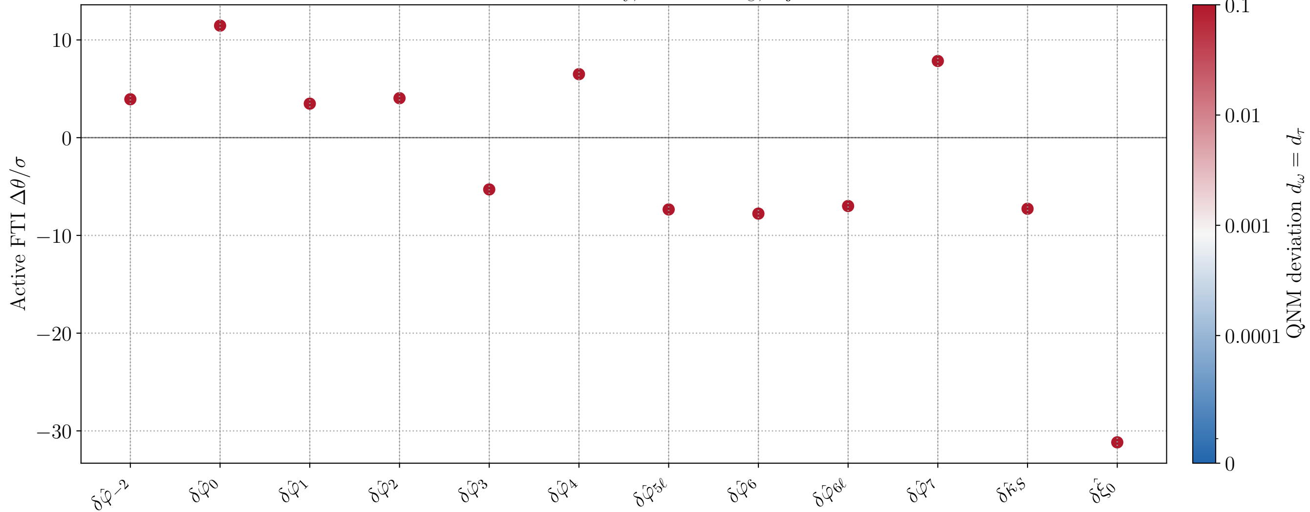
Active-FTI bias summary, M = 10^6 M_\odot , inj_id=0
