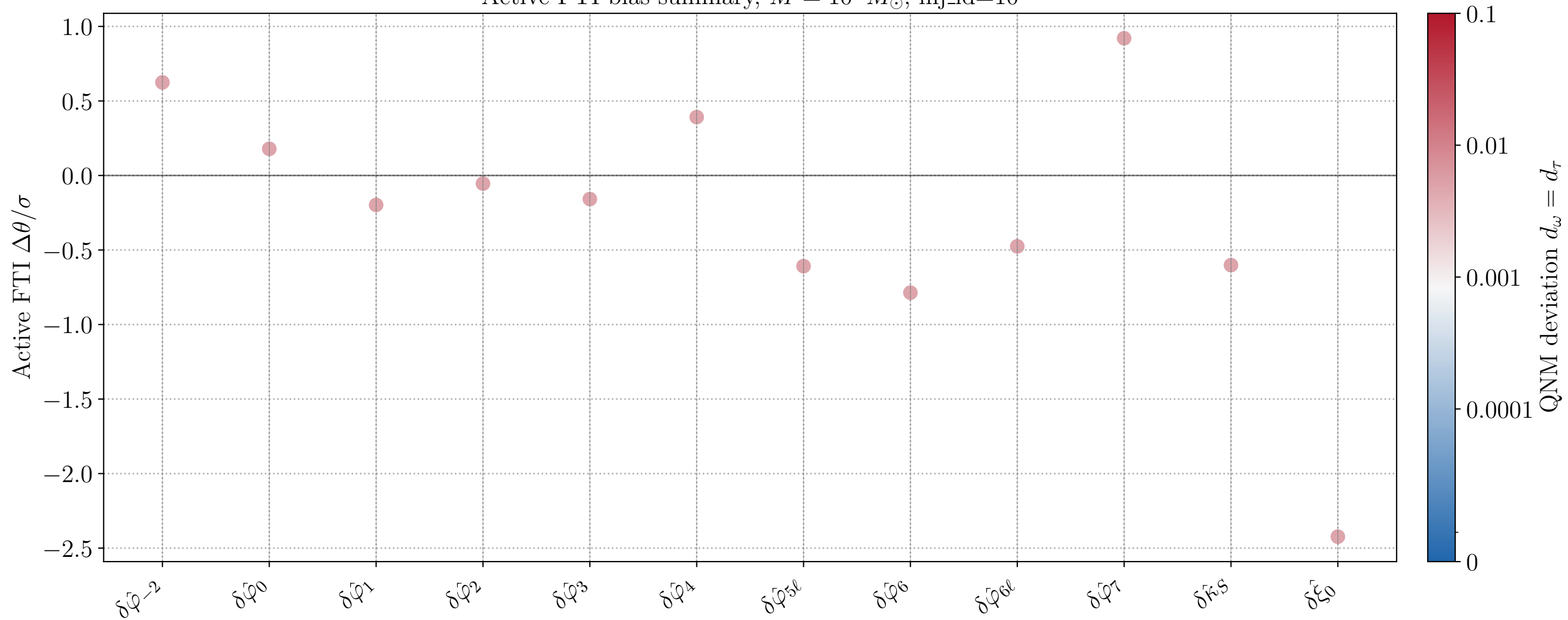
Active-FTI bias summary, M = 10^6 M_\odot , inj_id=10
