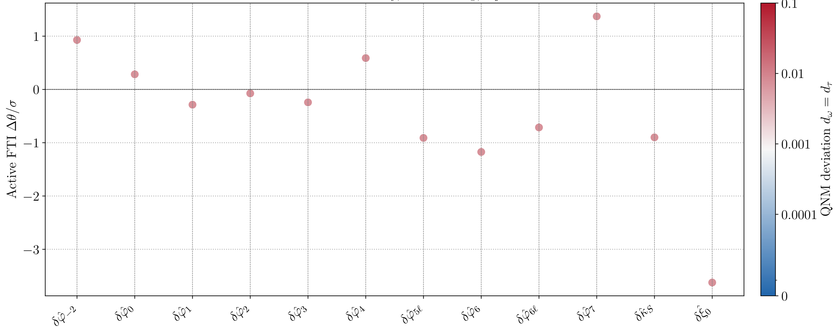
Active-FTI bias summary, M = 10^6 M_\odot , inj_id=11
